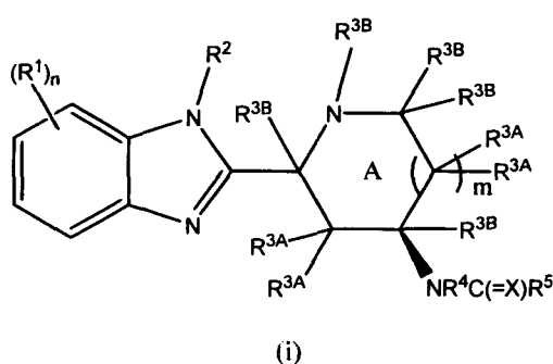
preferred stereochemistry
