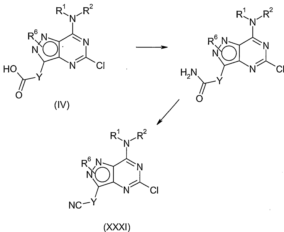
Scheme 29
