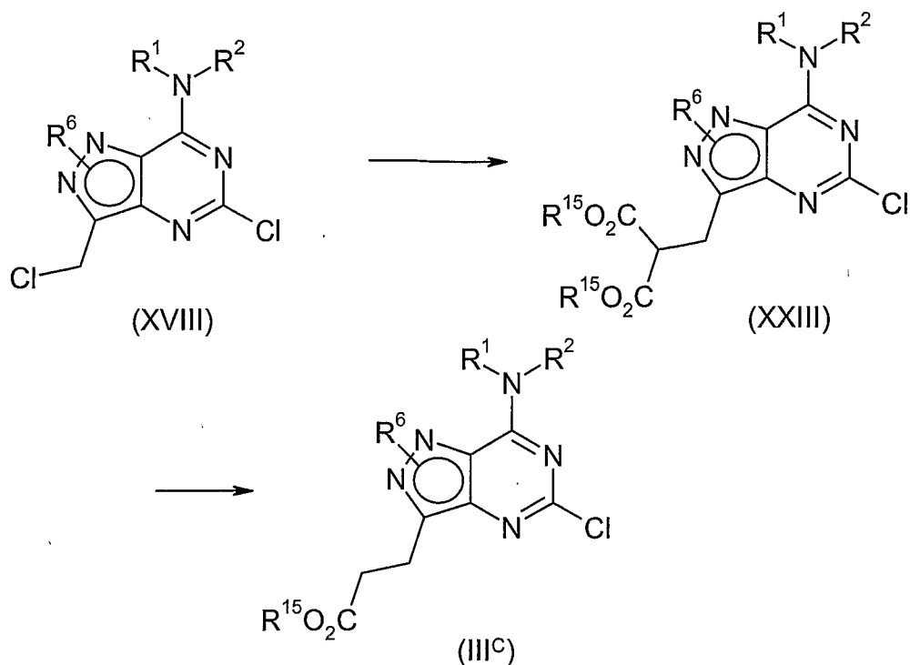
Scheme 24
