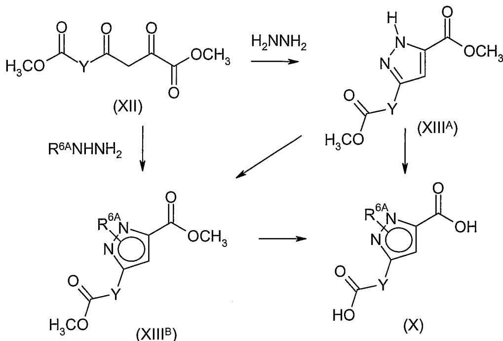
Scheme 12
