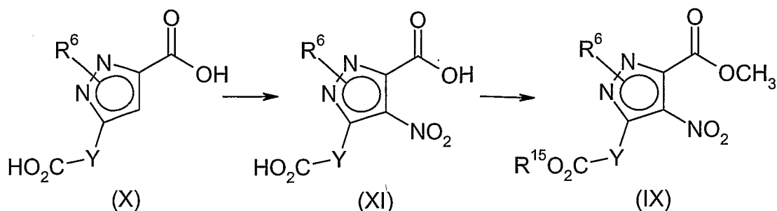
Scheme 11
