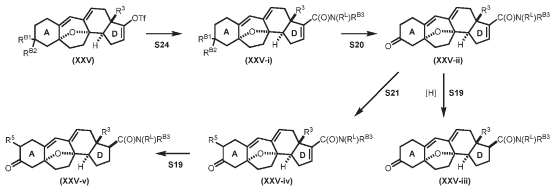
Scheme 11.
