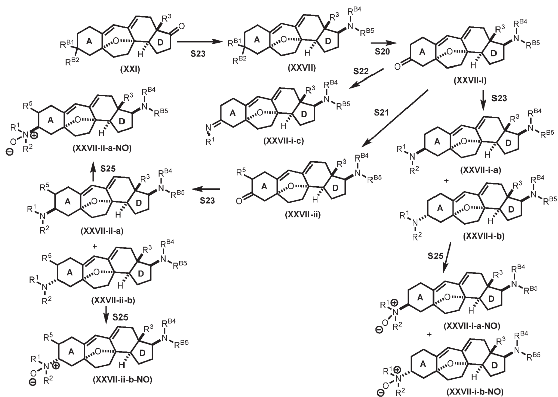
Scheme 13.
