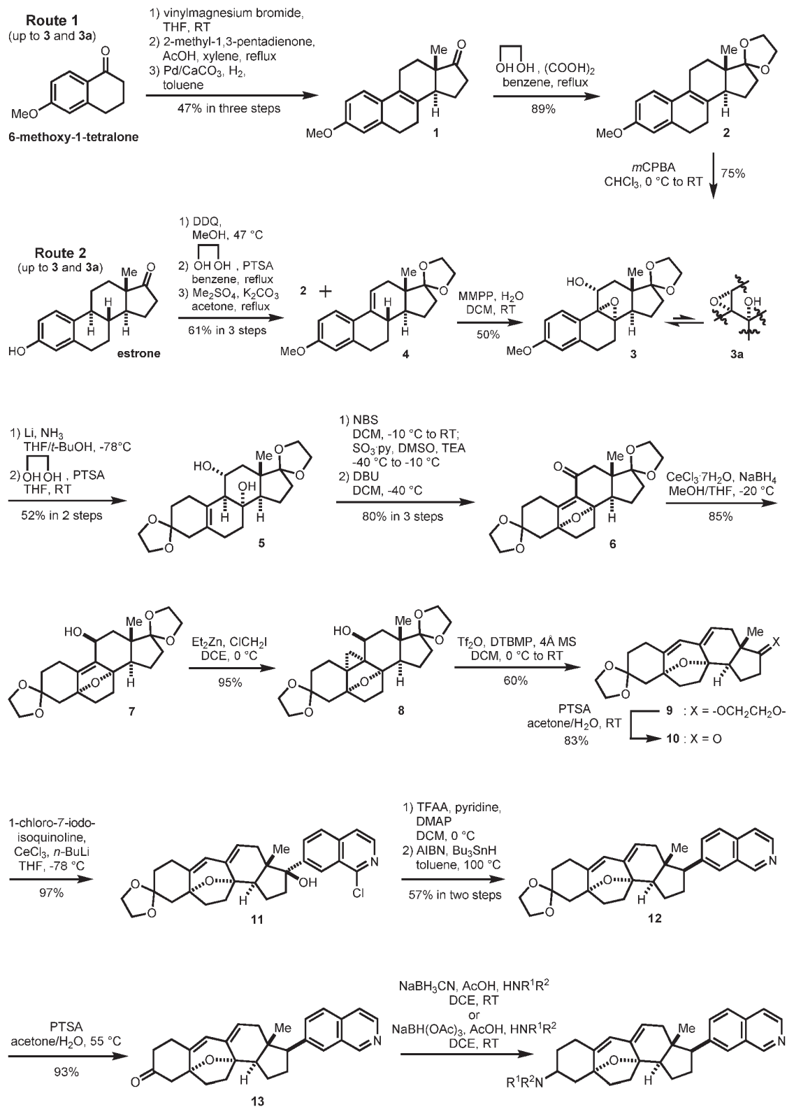
Scheme 1-1.
