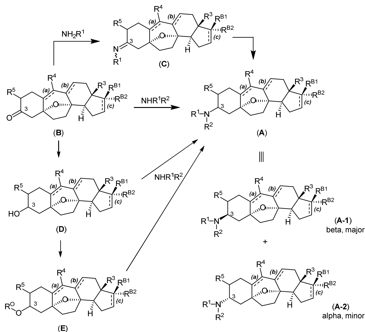
Scheme 1.
