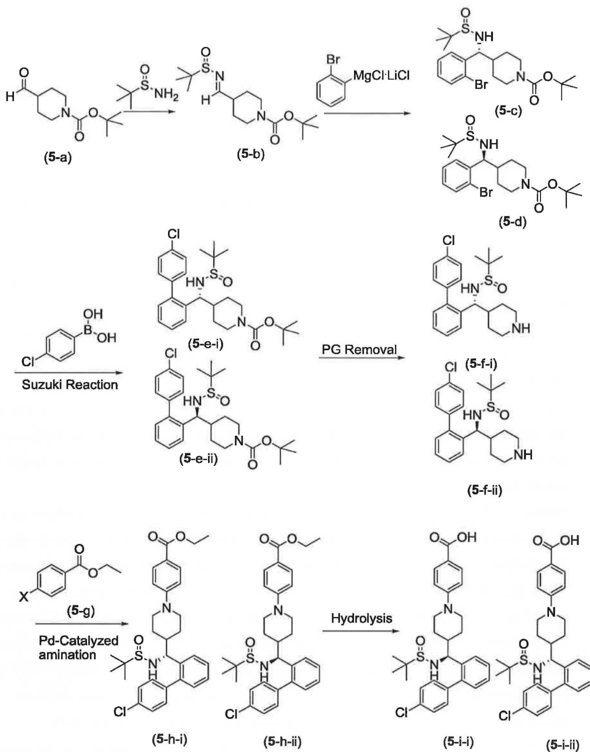
SCHEME 5
