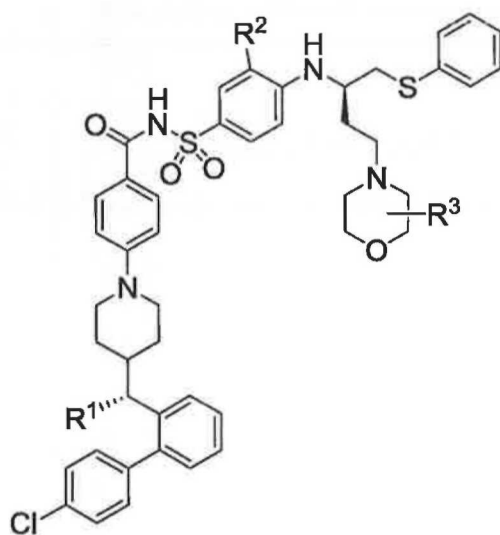
Formula (I-d)
