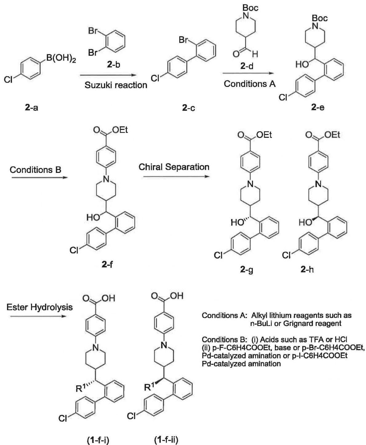
SCHEME 2
