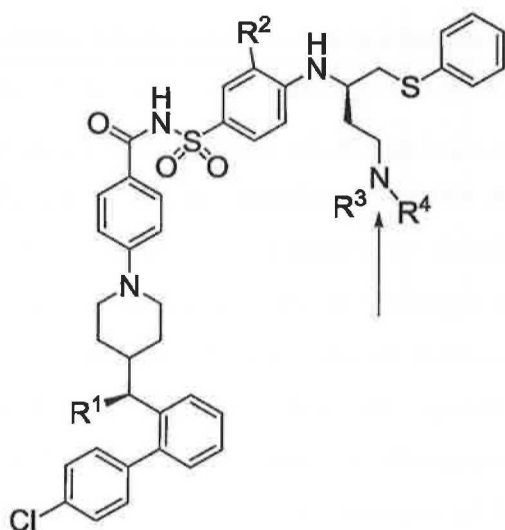
Formula (I-a)
