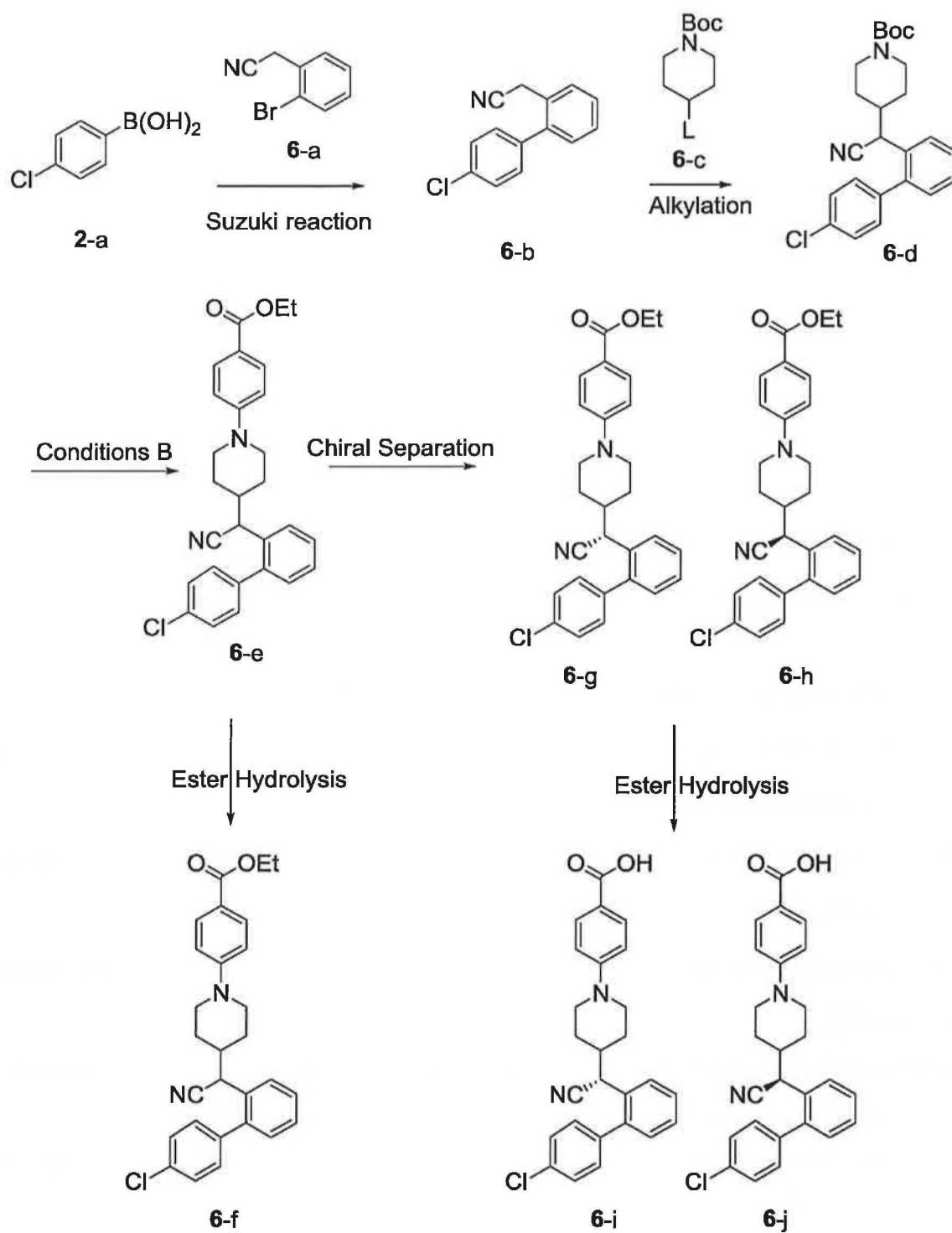
SCHEME 6
