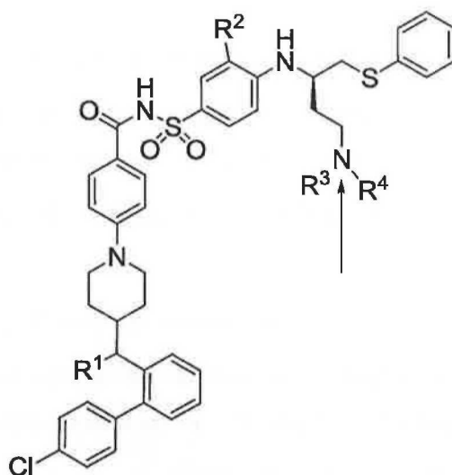
Formula (I)
