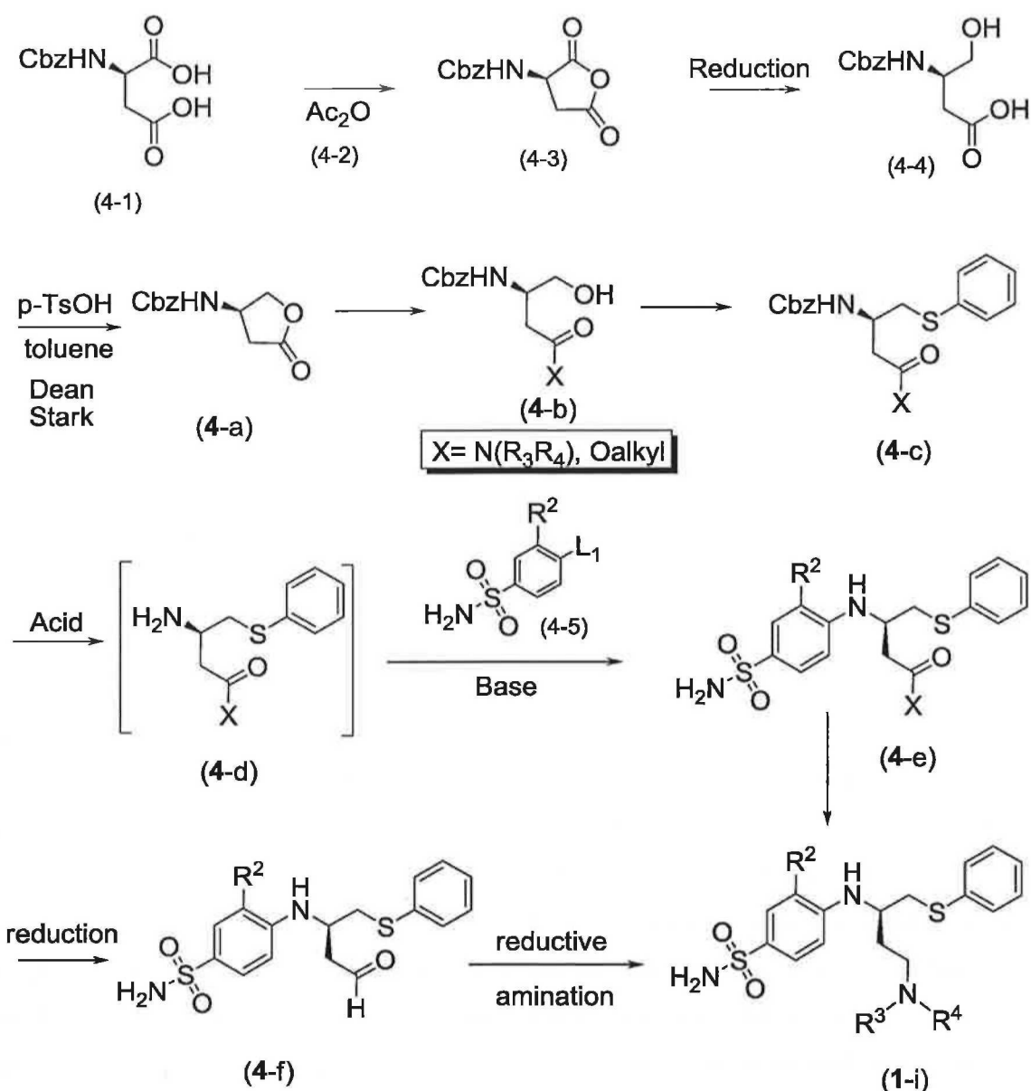
SCHEME 4
