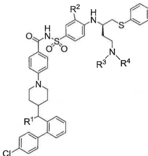
Formula (I)
