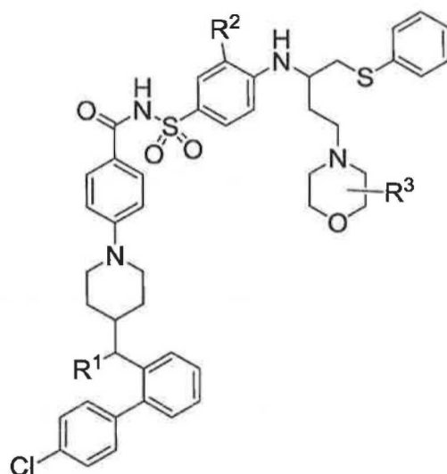
Formula (I-c)
