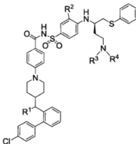
Formula (I)
