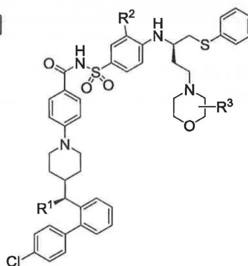
Formula (I-e)
