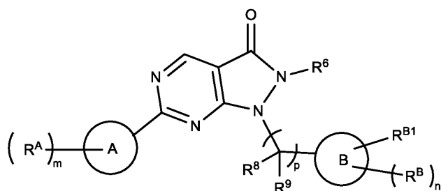
Formula (II e ).
