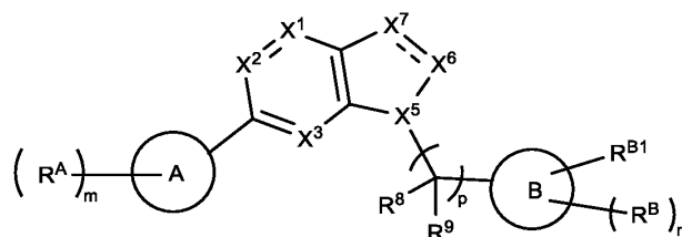
Formula (II').
