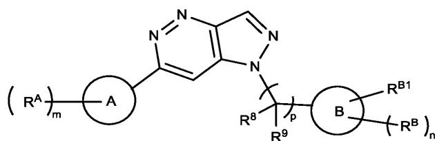
Formula (IIg).
