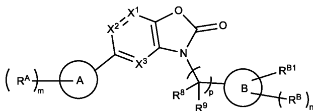
Formula (IIb).
