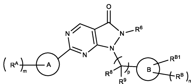
Formula (IIe).
