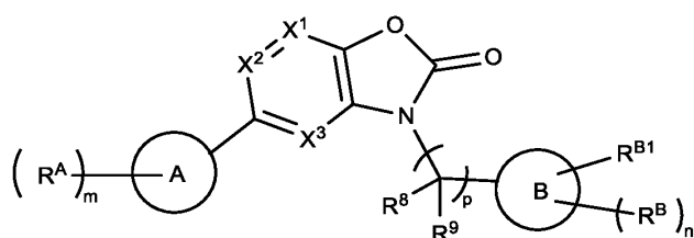
Formula (IIb).
