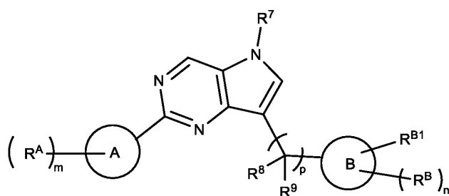
Formula (IIf).
