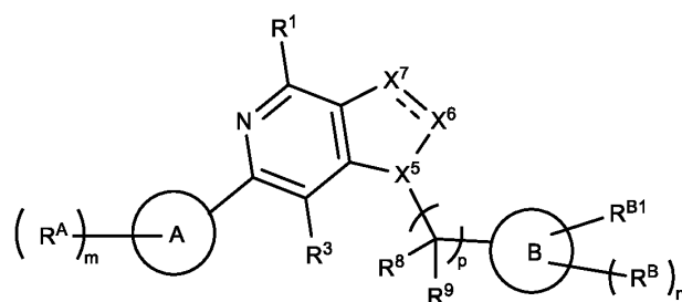
Formula (IIc').
