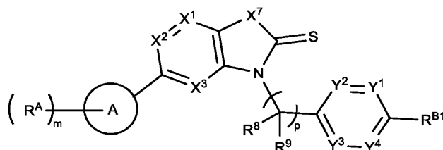
Formula (IIa-1),
