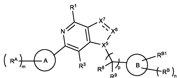
Formula (IIc').
