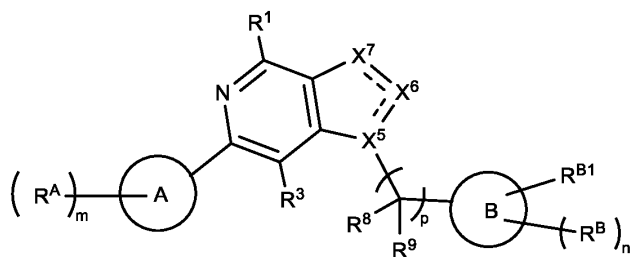
Formula (IIc).
