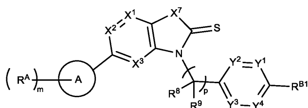
Formula (IIa-1),
