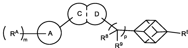
Formula (VI)
