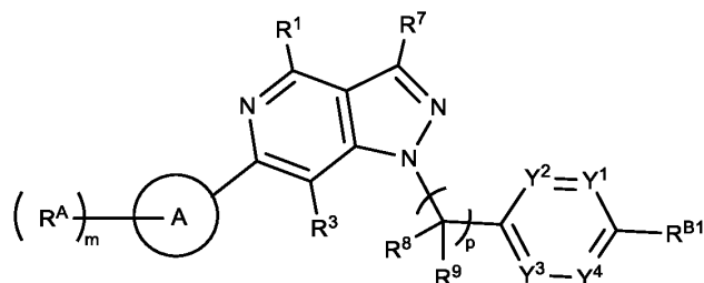
Formula (IIc-1),
