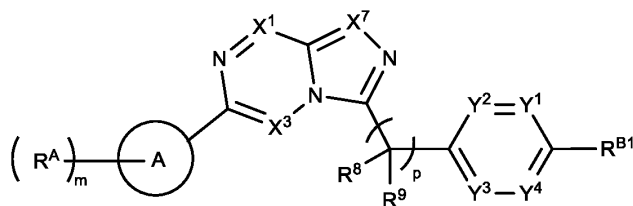
Formula (Ia)
