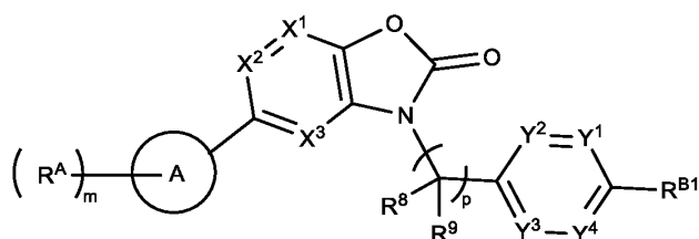
Formula (IIb-1)
