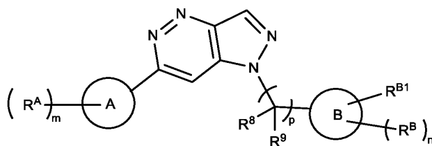
Formula (IIg).
