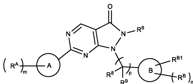
Formula (IIe).
