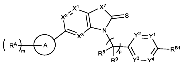
Formula (IIa-1)
