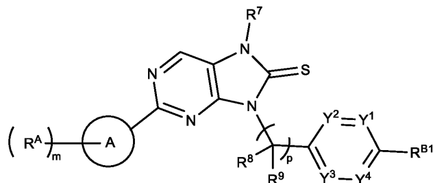
Formula (IIa-1a).
