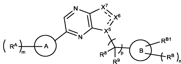
Formula (IIId).
