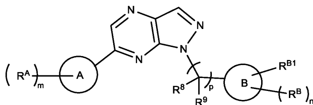
Formula (IIId-1).
