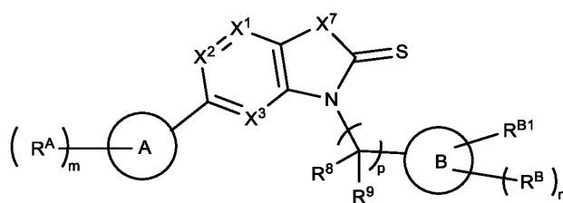
Formula (IIa).
