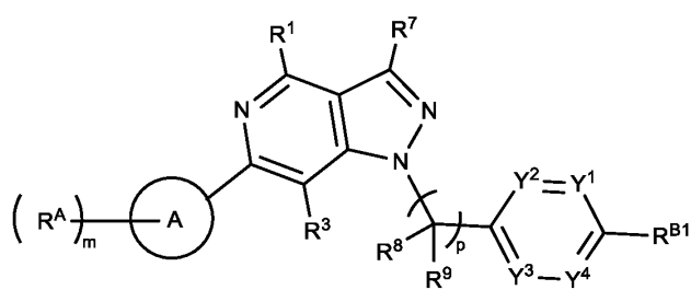
Formula (IIc-1),
