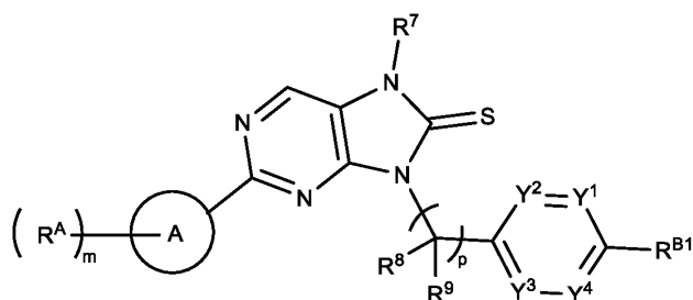
Formula (IIa-1a).
