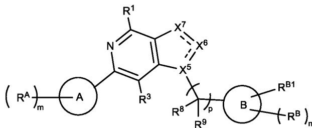
Formula (IIc).
