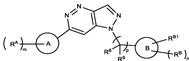
Formula (II g ).
