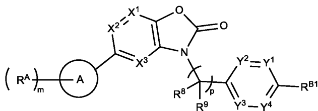
Formula (IIb-1),
