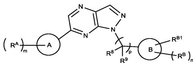
Formula (IId-1).
