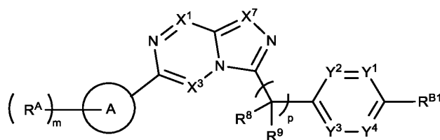
Formula (Ia)
