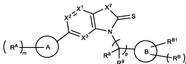
Formula (IIa).
