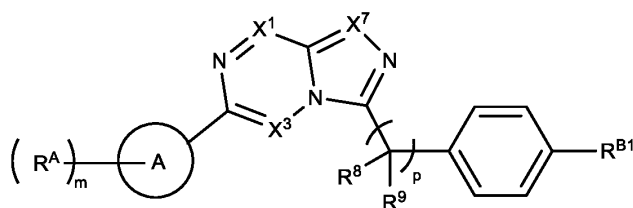
Formula (Ib).
