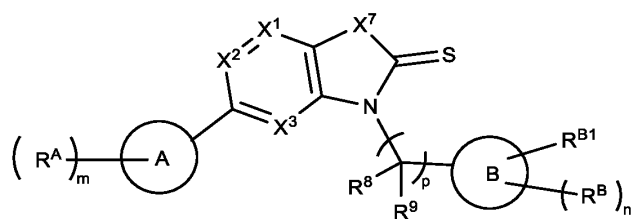
Formula (IIa)
