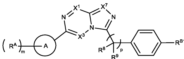
Formula (Ib).
