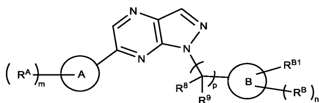
Formula (II d -1).
