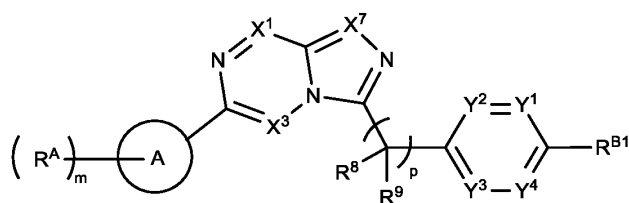
Formula (Ia)
