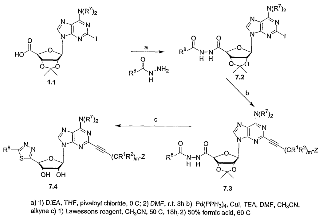
Scheme 7: Preparation of 4'-1,3,4 thiadiazole
