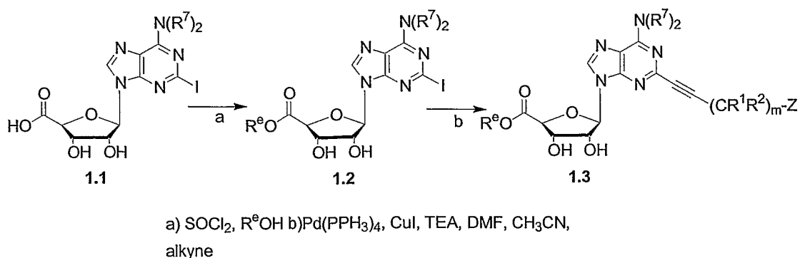
Scheme 1: Preparation of 5' ester analogs:
