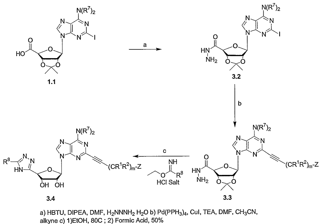
Scheme 3: Preparation of 4' triazoles:
