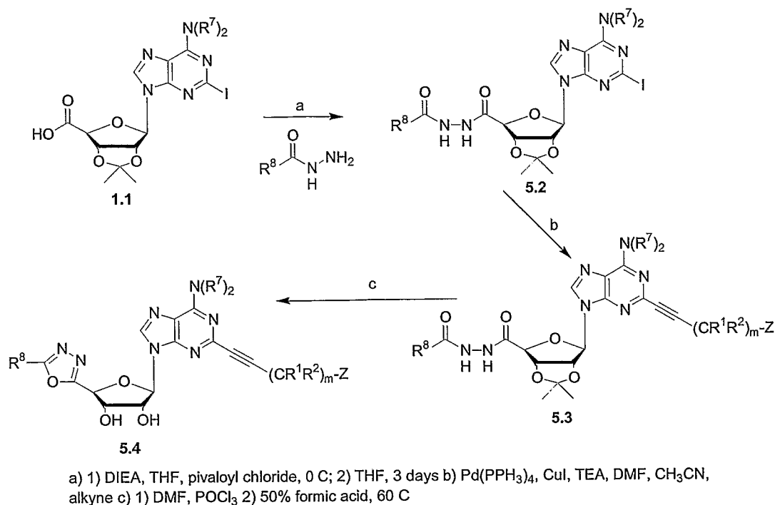
Scheme 5: Preparation of 4'-1,3,4 oxadiazoles
