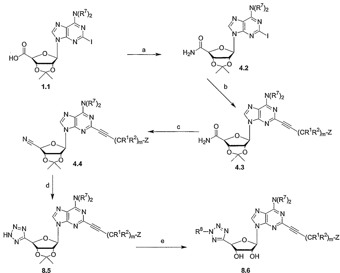
Scheme 8: Preparation of 4'-tetrazole
