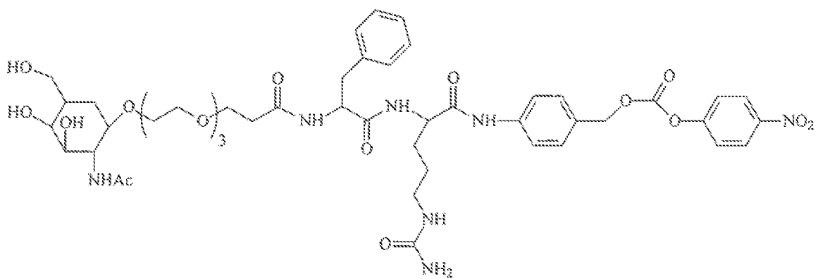
NAG-PEG4-PheCit-PABC-PNP
