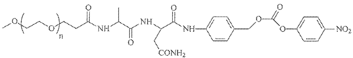
PEG-AlaAsn-PABC-PNP
