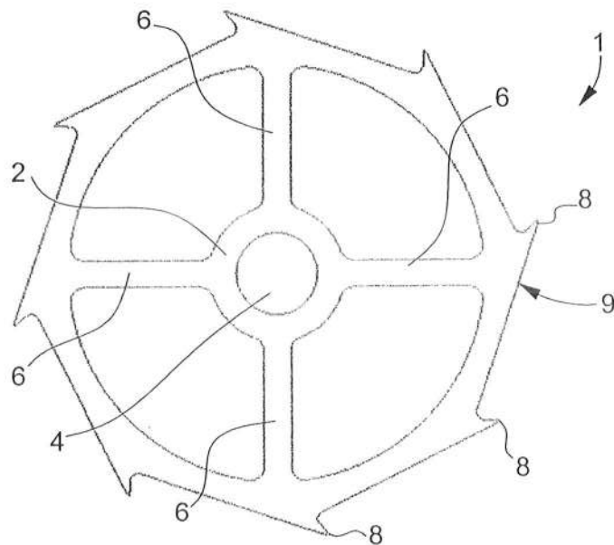
Fig. 2 ( Prior art )
