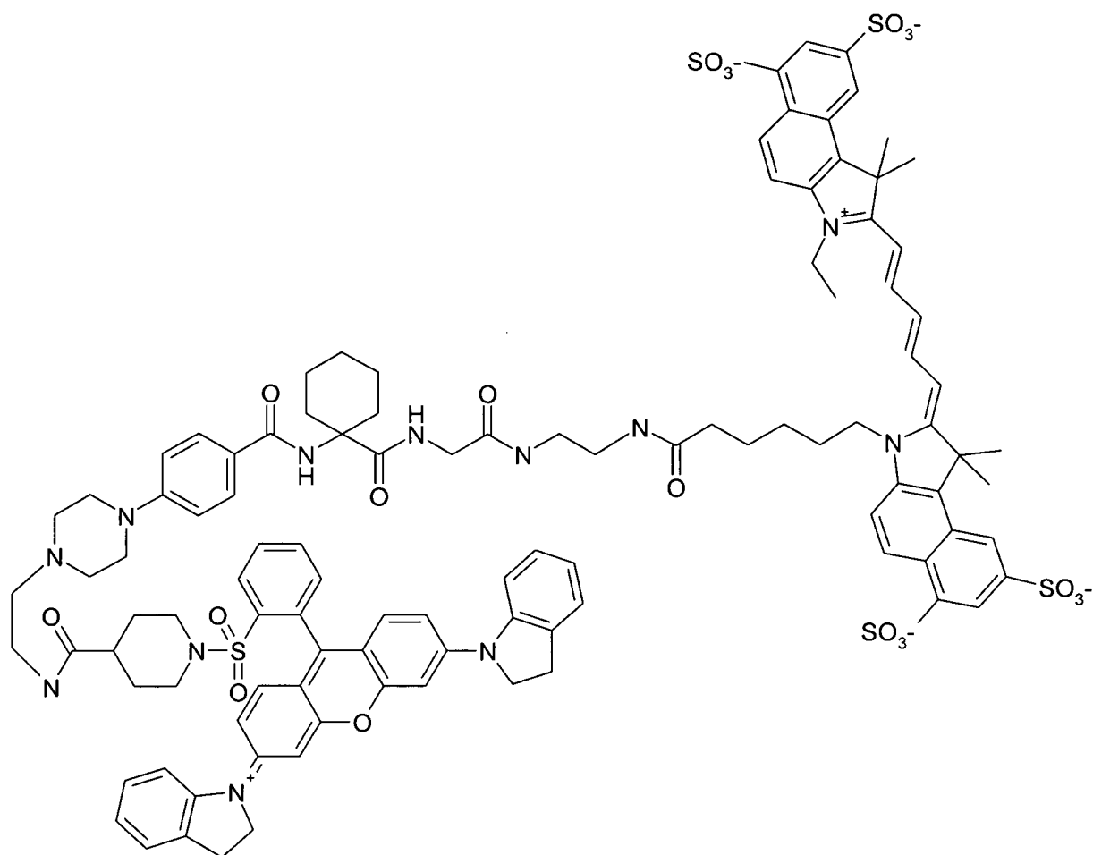
(Scheme 10)
