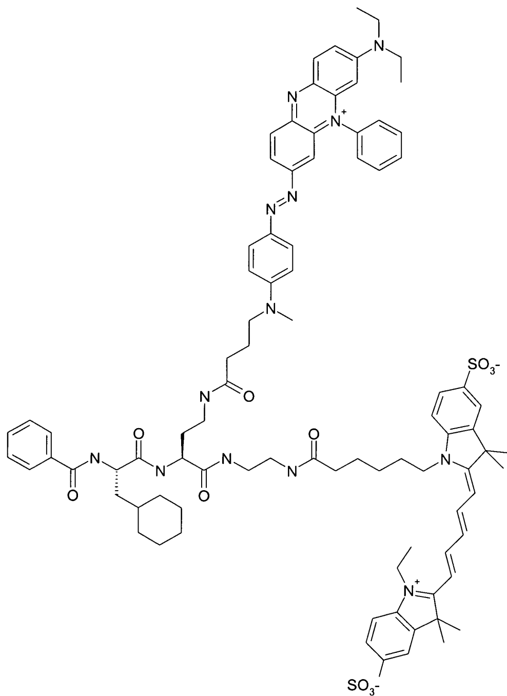
(Scheme 6)
