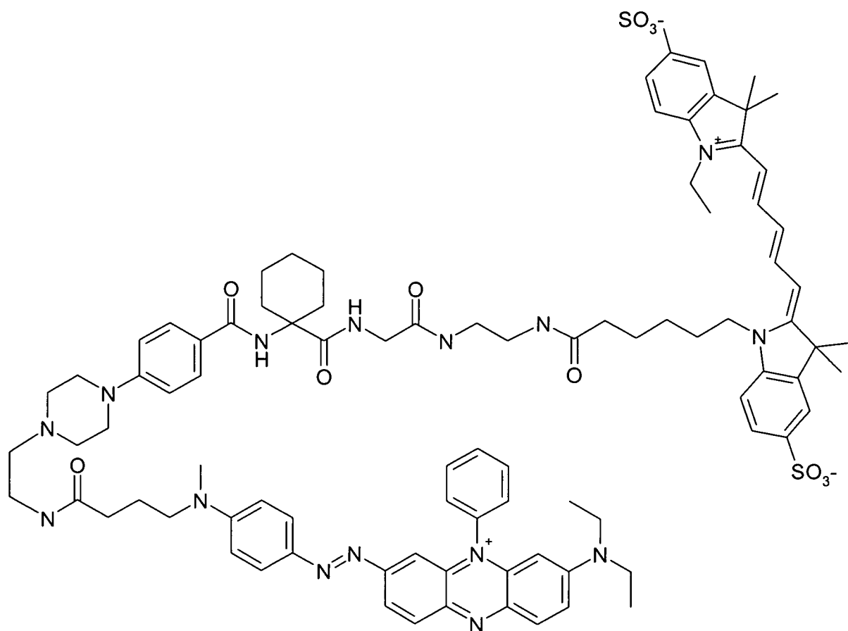
(Scheme 11)
