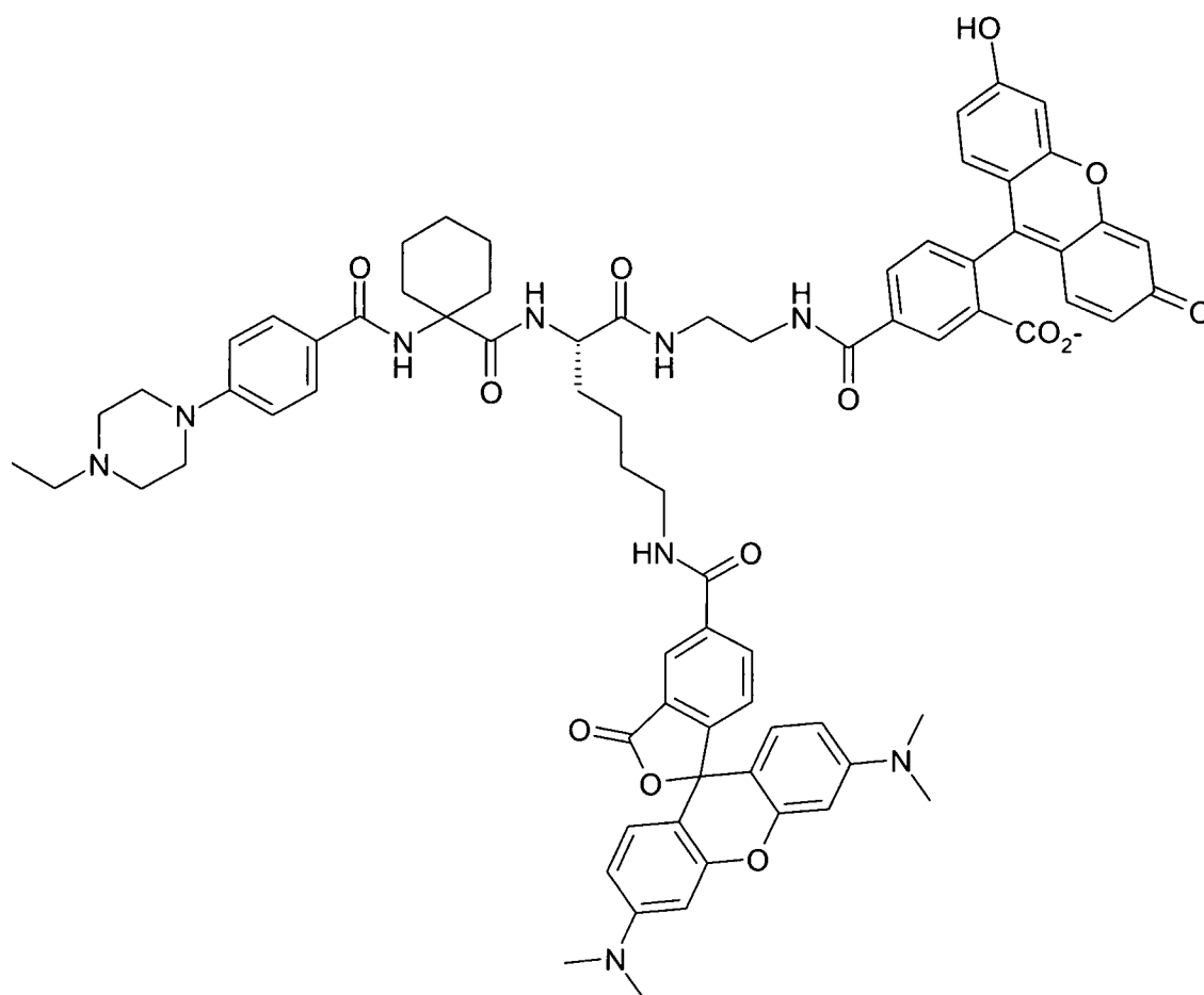
(Scheme 8)
