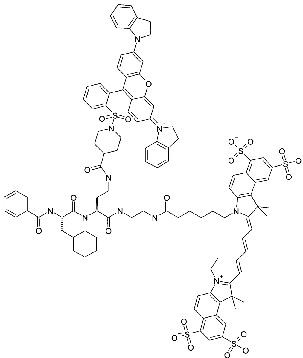
(Scheme 4)
