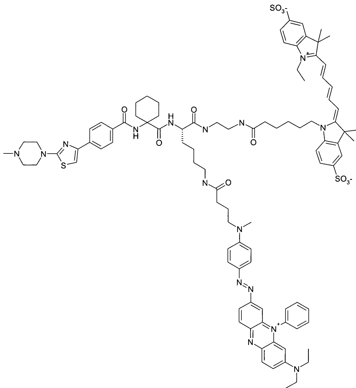
(Scheme 13)
