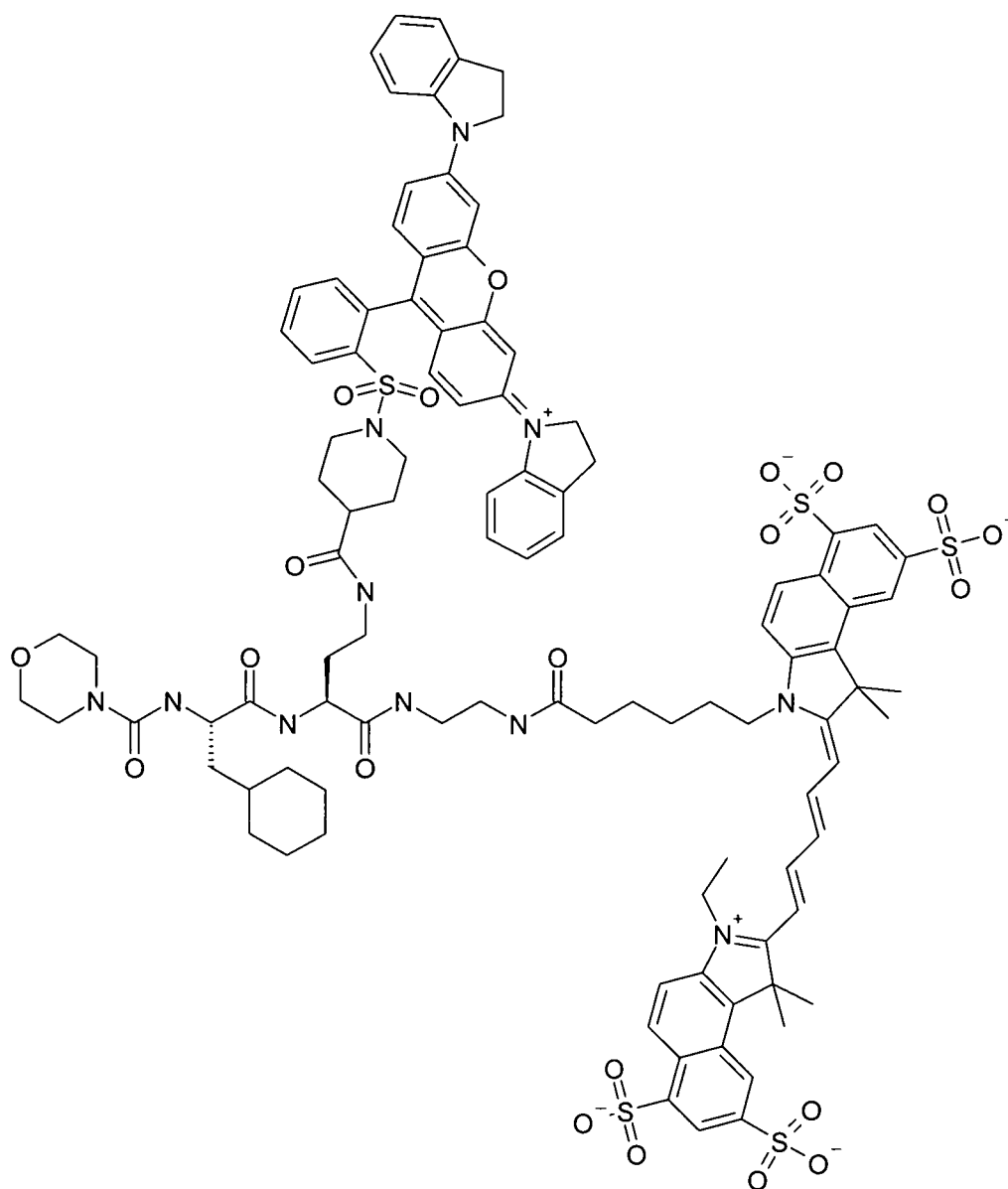
(Scheme 2)
