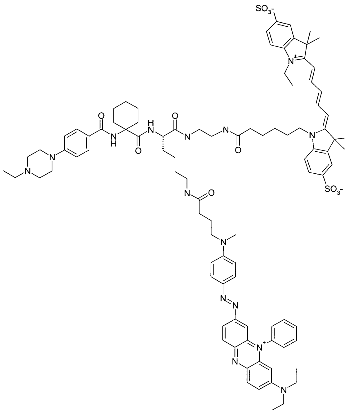
(Scheme 9)
