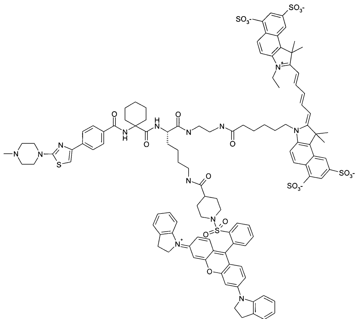
(Scheme 12)
