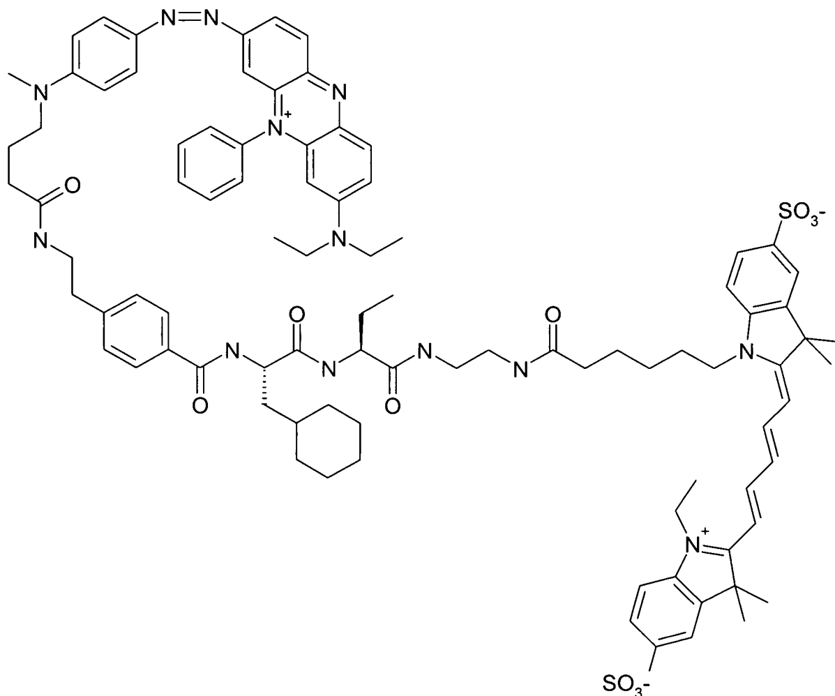
(Scheme 7)
