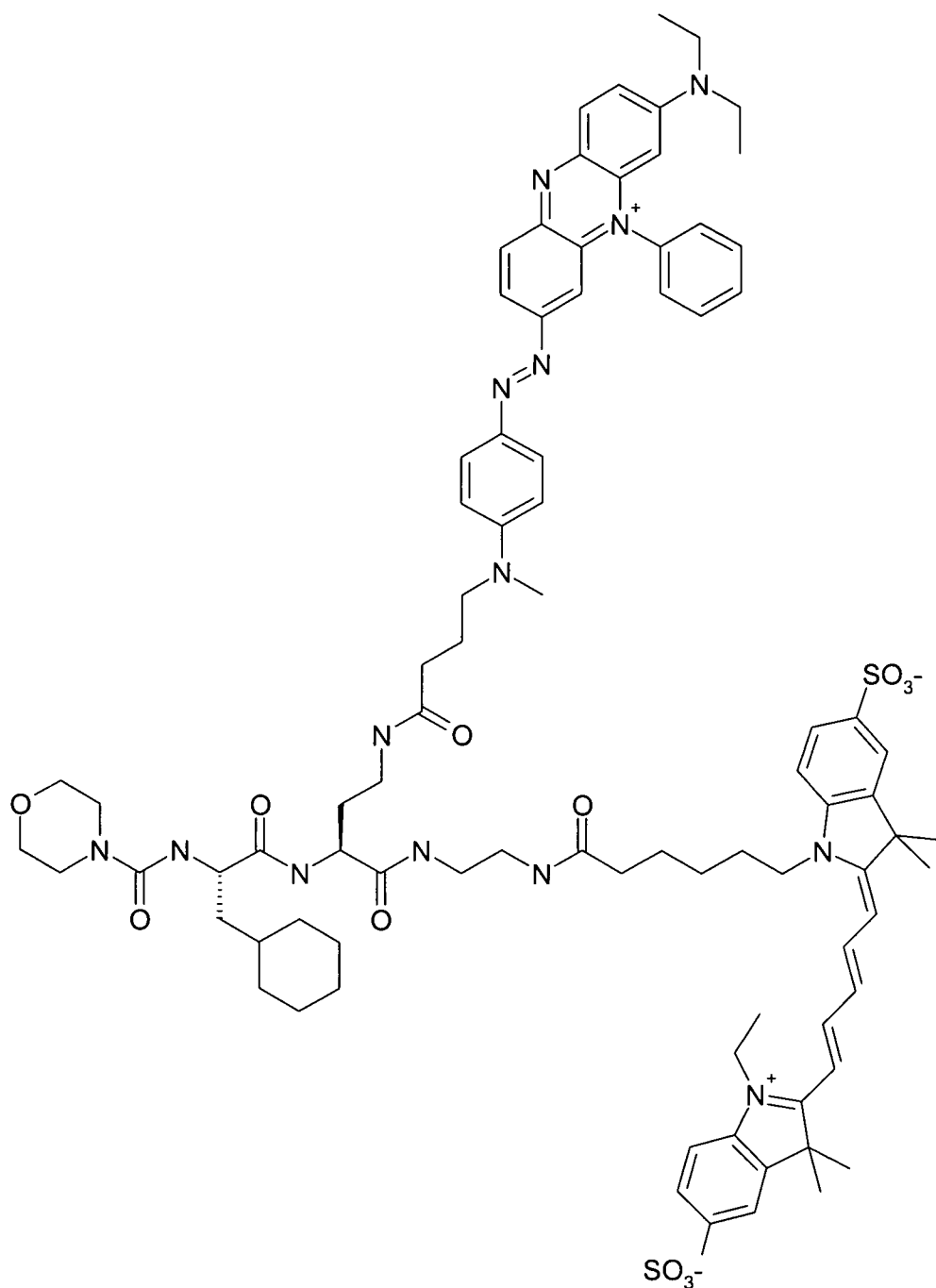
(Scheme 3)
