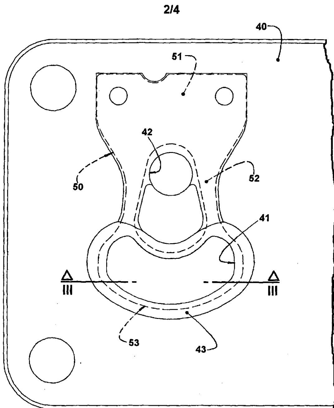
FIG. 2 PRIOR ART
