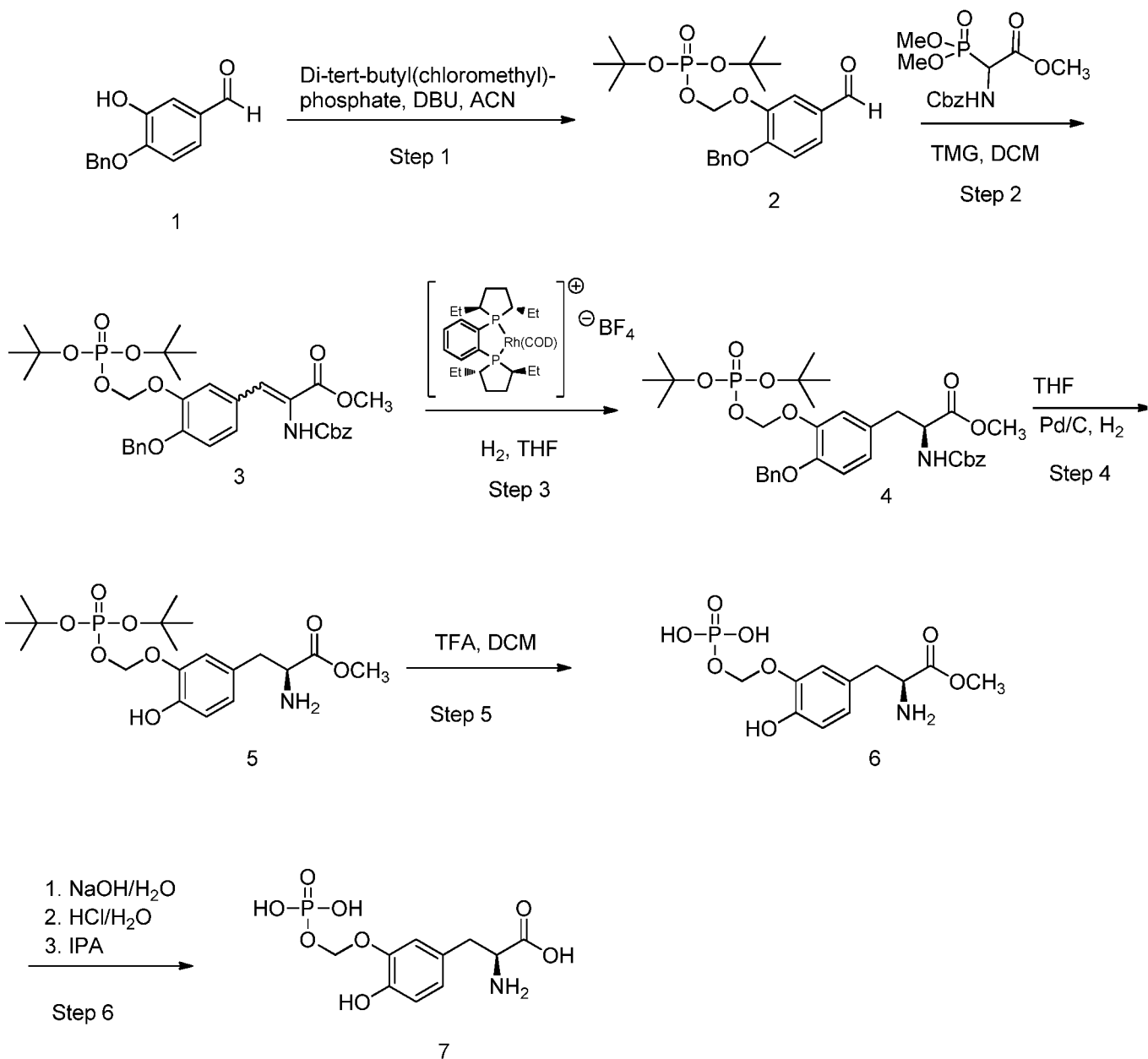
Scheme 8
