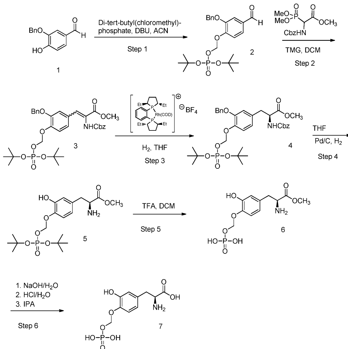
Scheme 9
