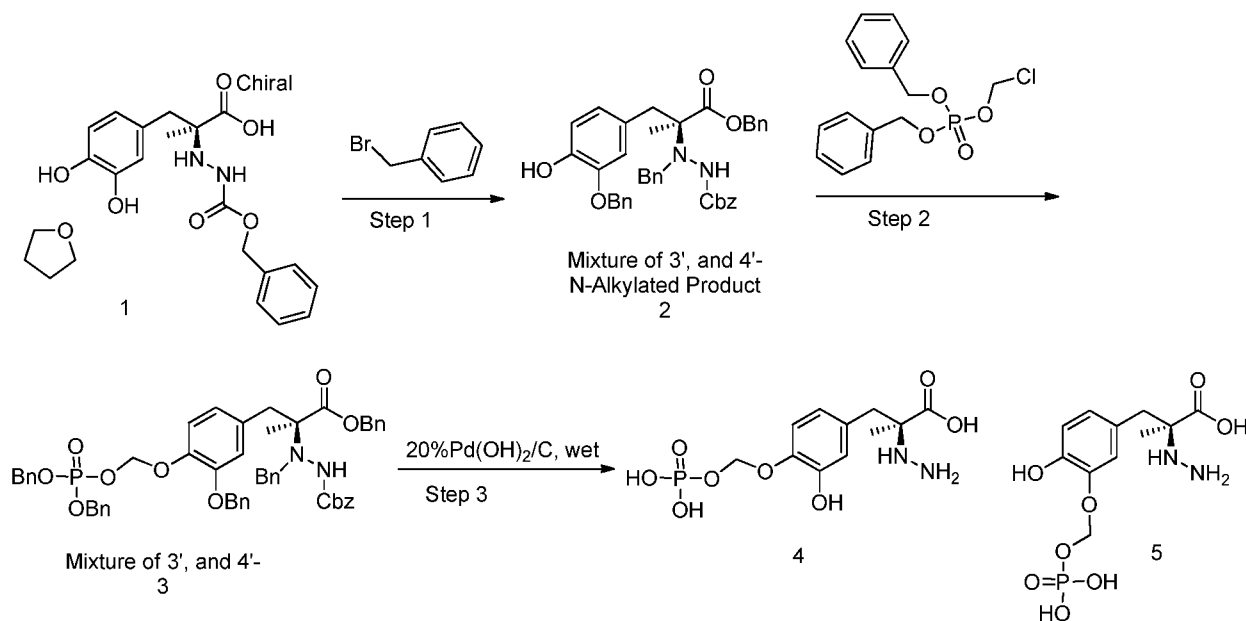
Scheme 10
