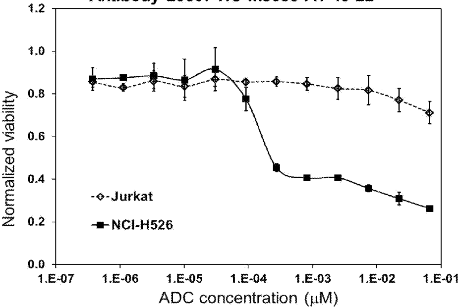
FIG. 2D Antibody 20507-HC-ins388-A1-49-22
