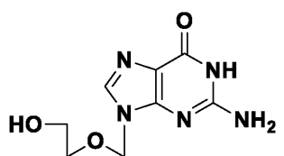
Acyclovir (ACV)
