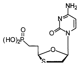
3'-thia-2',3'- dideoxycytidine-5'- phosphonic acid
