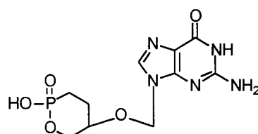
Ganciclovir cyclic phosphonate
