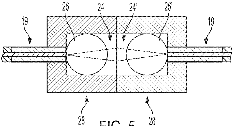
FIG. 5 PRIOR ART
