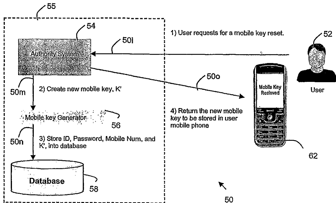
Figure 6. Mobile key reset process
