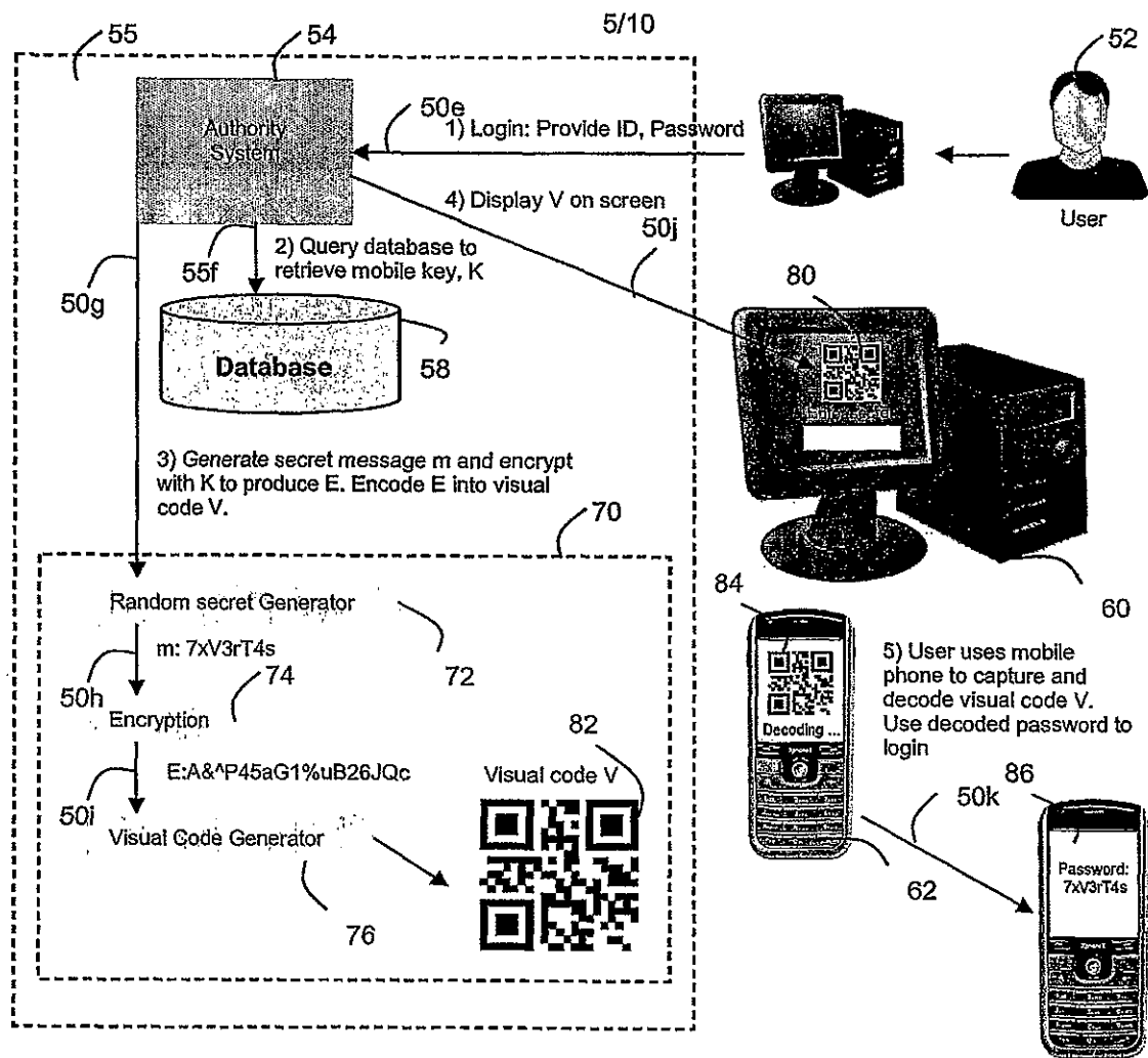
Figure 5. User login process
