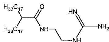
GUADACA (Guanidino-DACA)
