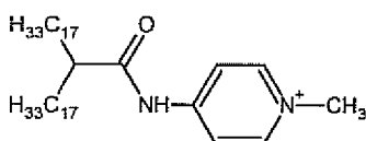
MPDACA (Methylpyridiyl-DACA)
