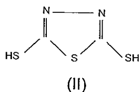
2,5-dimercapto-1,3,4-thiadiazole
