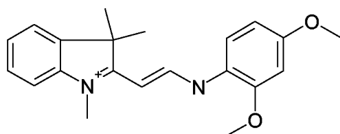
Cation of Basic Yellow 11
