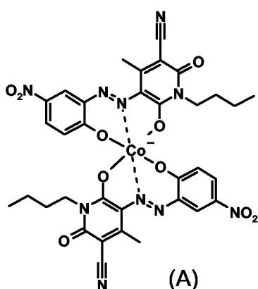
Azo metal Complex A
