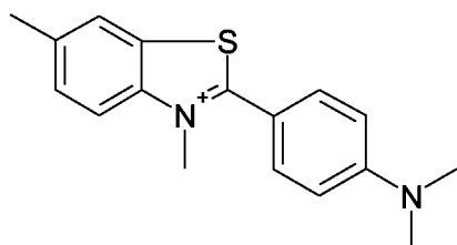
Cation of Basic Yellow 1
