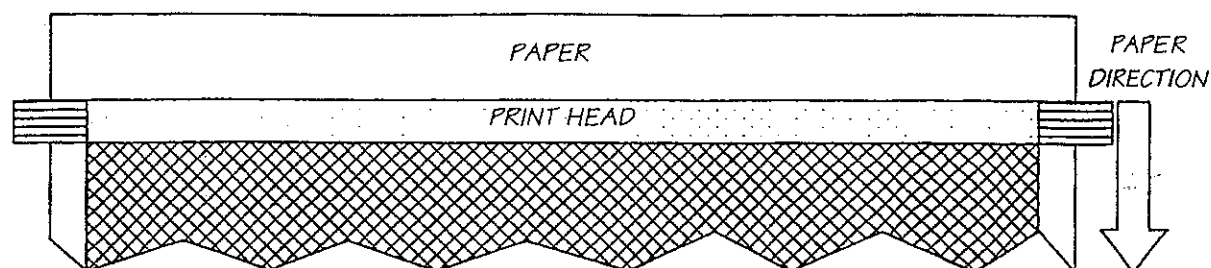
8 PRINT HEAD SEGMENTS IN PRINT HEAD
