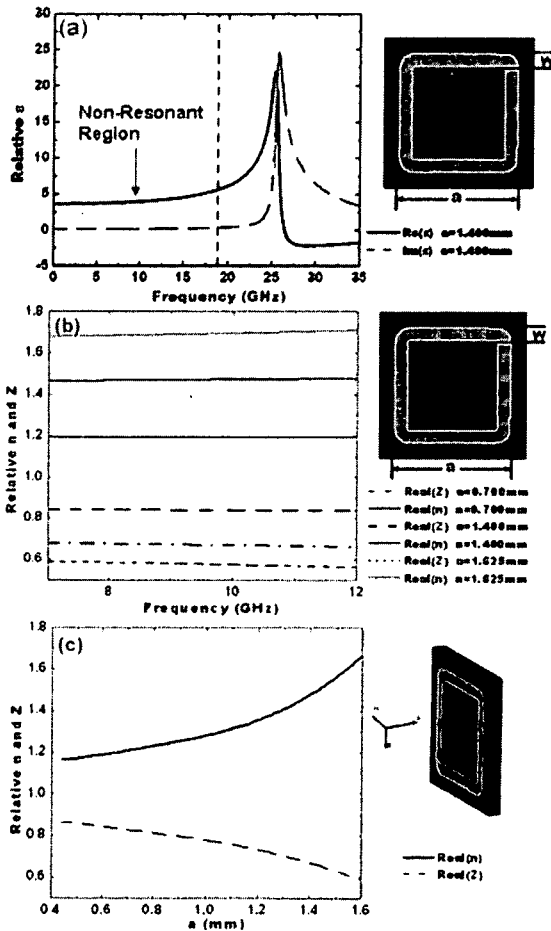
Fig. 2. (Color online) Retrieval results for the closed ring medium. In all cases the radius of curvature of the corners is 0.6 mm, and w=0.2 mm. (a) The extracted permittivity with a=1.4 mm. (b) The extracted index and impedance for several values of a . The low frequency region is shown. (c) The relationship between the dimension a and the extracted refractive index and wave impedance.
