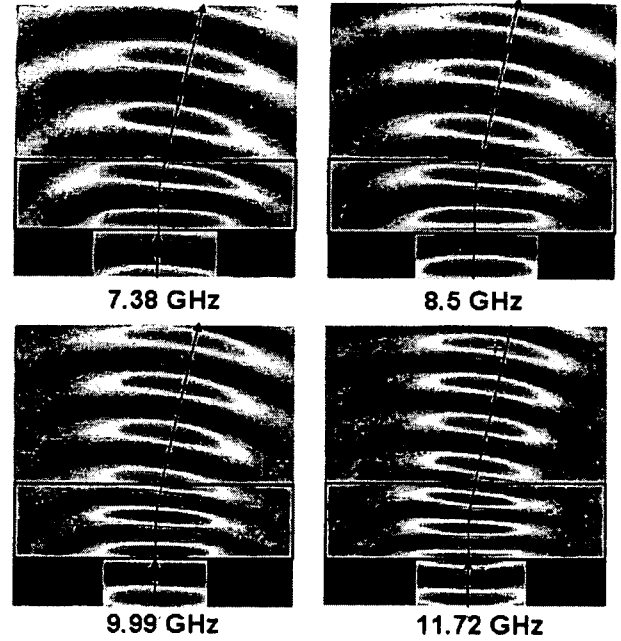
Fig. 5. Field mapping measurements of the beam steering lens. The lens has a linear gradient that causes the incoming beam to be deflected by an angle of 16.2 degrees. The effect is broadband, as can be seen from the identical maps taken at four different frequencies that span the X-band range of the experimental apparatus.
