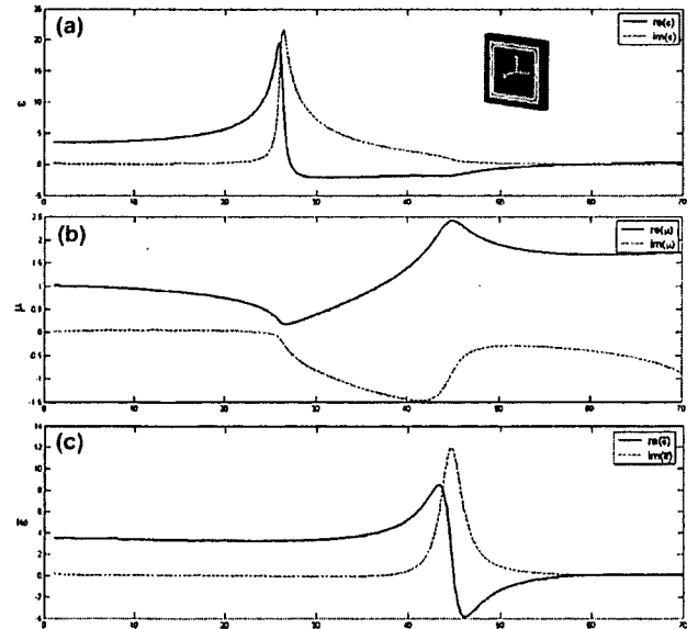
Fig. 1. (a) Retrieved permittivity for a metamaterial composed of the repeated unit cell shown in the inset; (b) retrieved permeability
