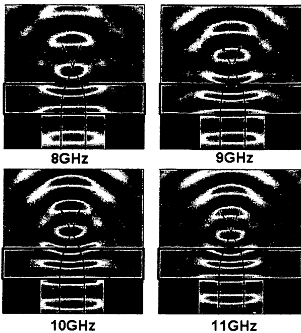
Fig. 6. Field mapping measurements of the beam focusing lens. The lens has a symmetric profile about the center (given in the text) that causes the incoming beam to be focused to a point. Once again, the function is broadband, as can be seen from the identical maps taken at four different frequencies that span the X-band range of the experimental apparatus.
