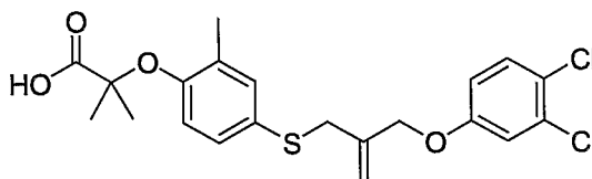
Compound 4
