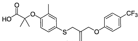
Compound 1
