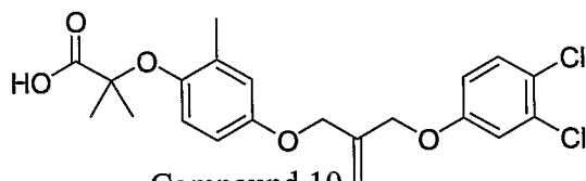
Compound 10
