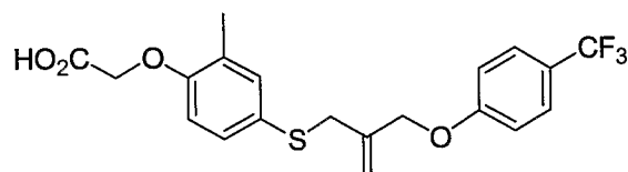
{2-Methyl-4-[2-(4-trifluoromethyl-phenoxy)methyl]-allylsulfanyl]-phenoxy}-acetic acid
