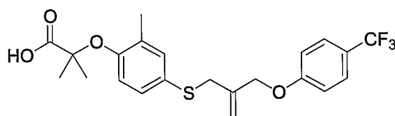
Compound 1
