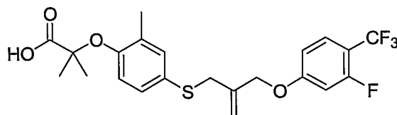
Compound 5
