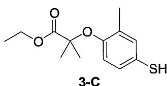
2-(4-Mercapto-2-methyl-phenoxy)-2-methyl-propionic acid ethyl ester
