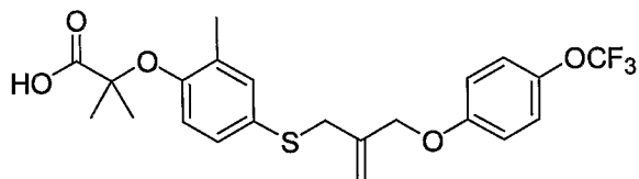
Compound 2
