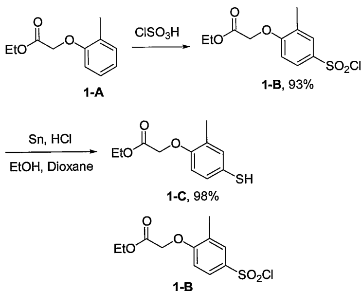
(4-Chlorosulfonyl-2-methyl-phenoxy)-acetic acid ethyl ester
