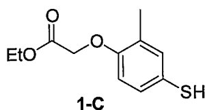
(4-Mercapto-2-methyl-phenoxy)-acetic acid ethyl ester
