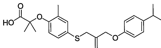
Compound 6
