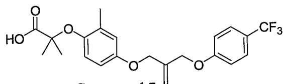
Compound 7
