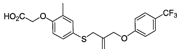
{2-Methyl-4-[2-(4-trifluoromethyl-phenoxy)methyl]-allylsulfanyl]-phenoxy}-acetic acid
