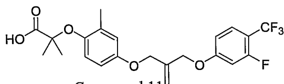
Compound 11
