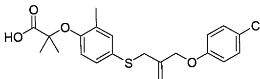
Compound 3
