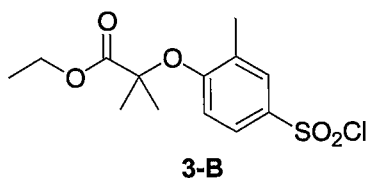
2-(4-Chlorosulfonyl-2-methyl-phenoxy)-2-methyl-propionic acid ethyl ester
