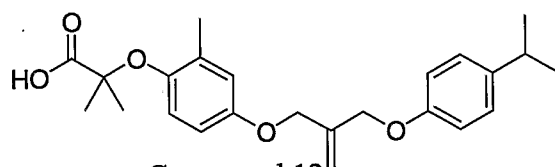
Compound 12
