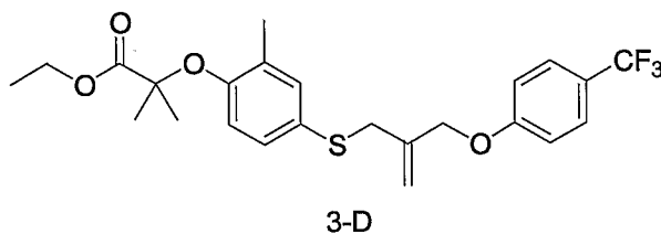
2-Methyl-2-{2-methyl-4-[2-(4-trifluoromethyl-phenoxy)methyl]-allylsulfanyl]-phenoxy}-propionic acid ethyl ester
