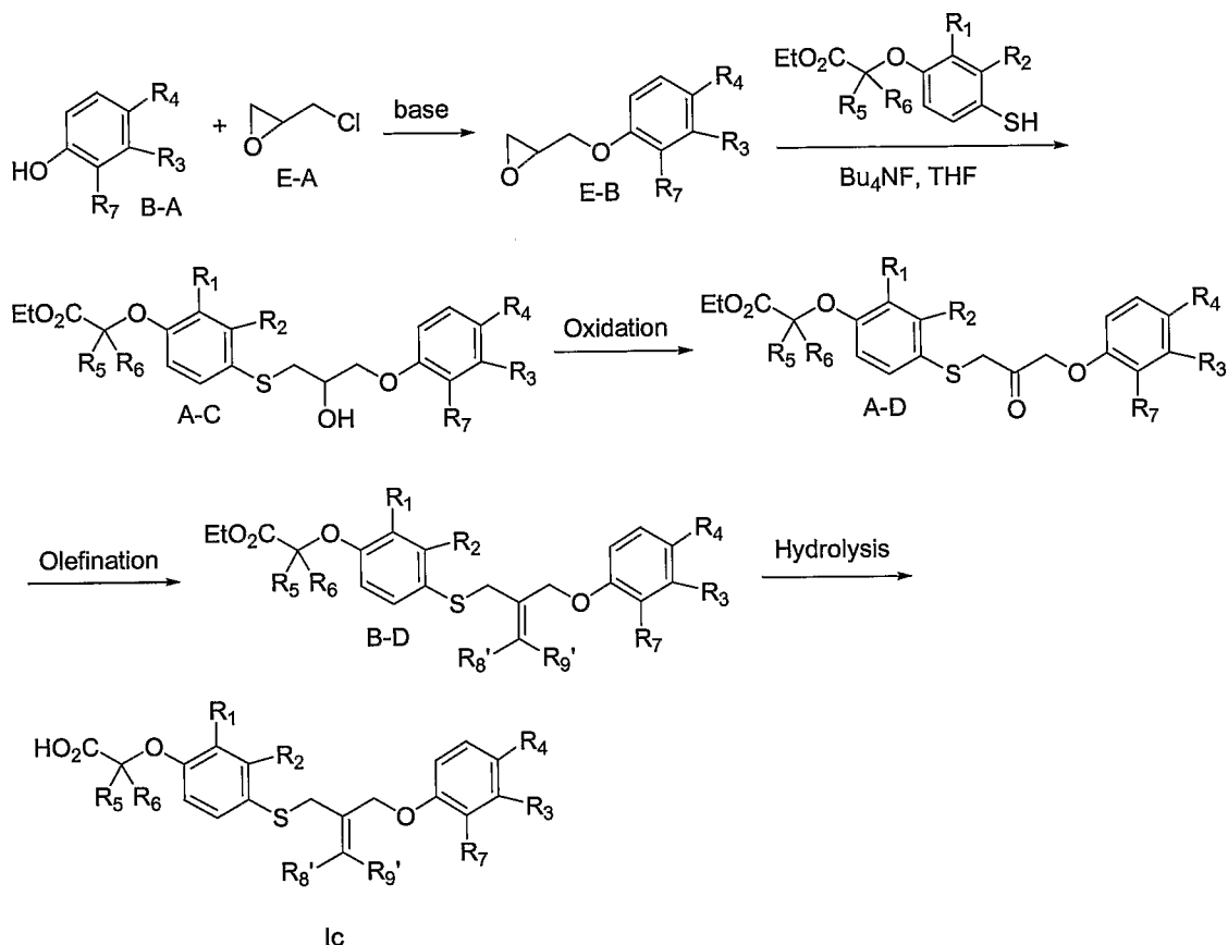
Scheme E
