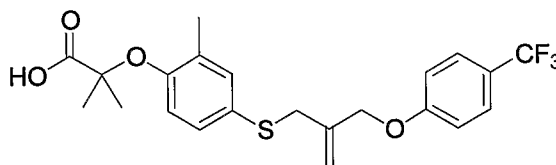
15 Compound 1, 47%
