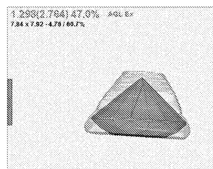
1.29ct round shape diamond polished from an inventive bipyramidal stone 47.0% polish yield
