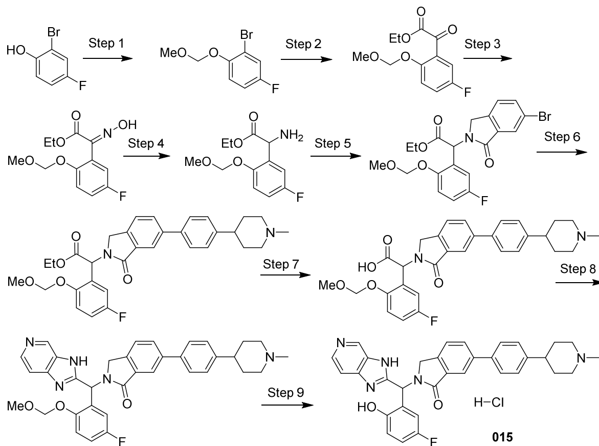
Scheme 2.
