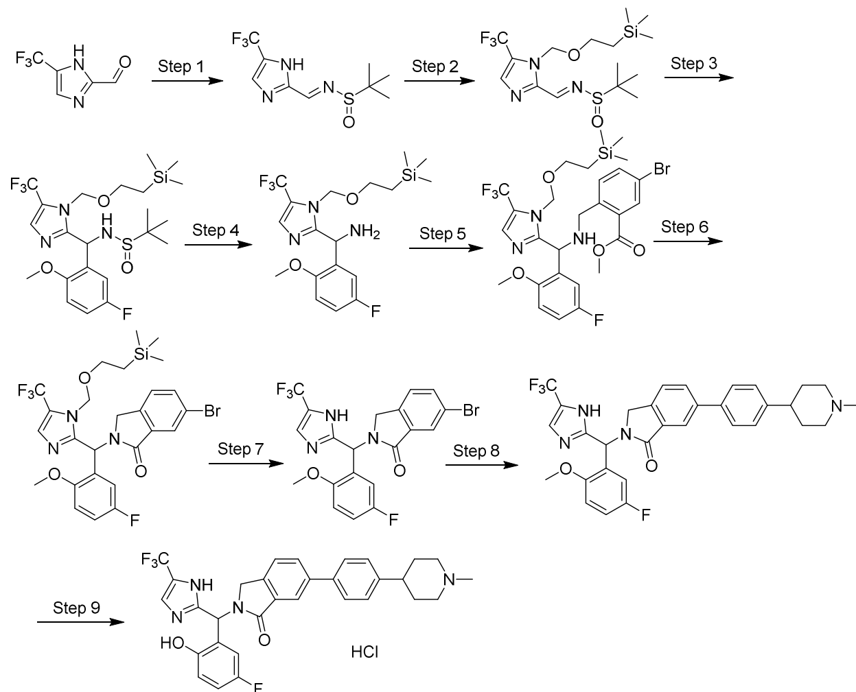
Scheme 21
