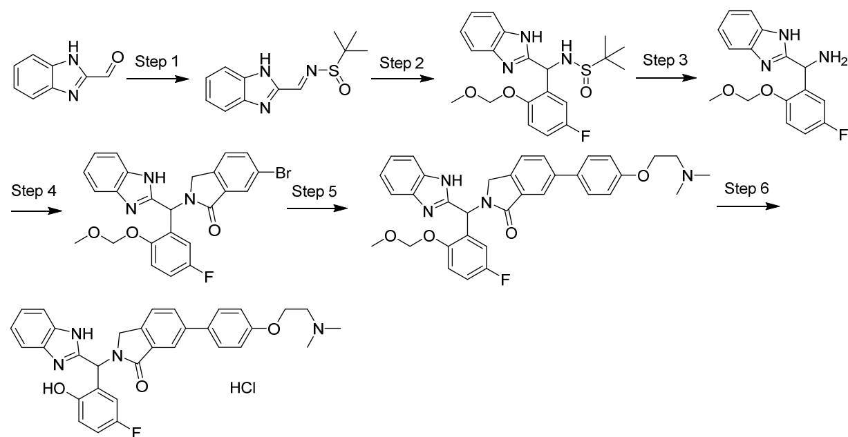
Scheme 17
