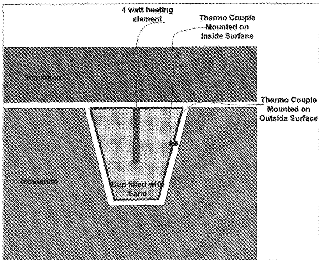
Thermal Resistance Test Assembly
