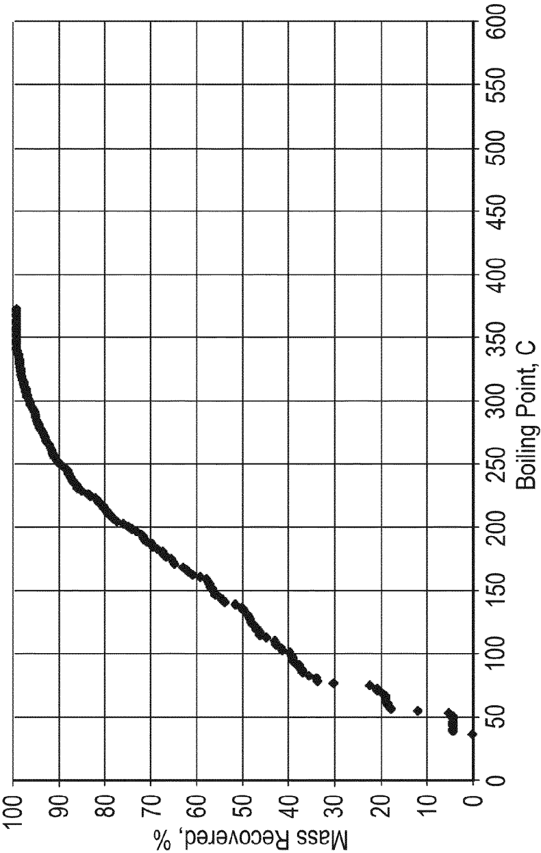
Fig.7 Example 3 SIMDIS Profile (ASTM D2887) for TPL-Hydrocarbon Product
