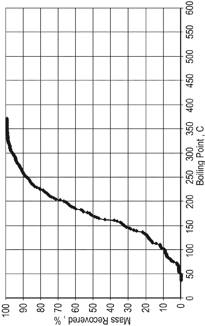
Fig.5 Example 2 SIMDIS Profile (ASTM D2887) for TPL-Hydrocarbon Product
