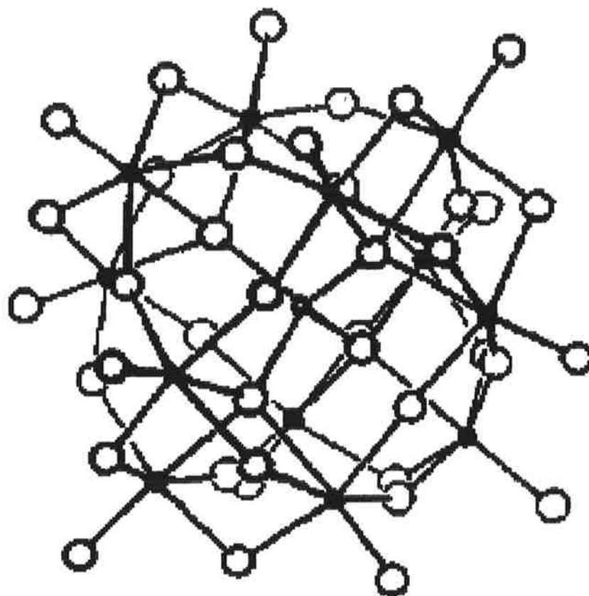
Figure 1: Structure of \text{XM}_{12}\text{O}_{40}
