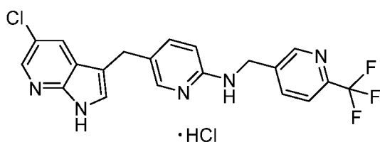
Compound I
