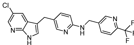
Compound II
