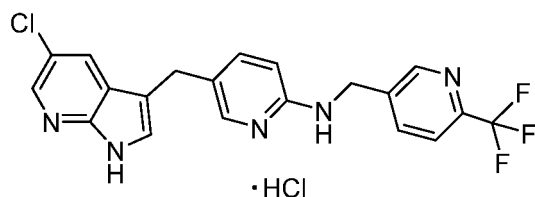
Compound I
