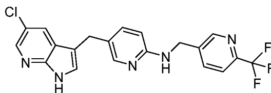
Compound II
