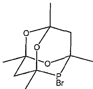
Compound CgPBr
