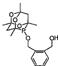
Compound CgP-OH
