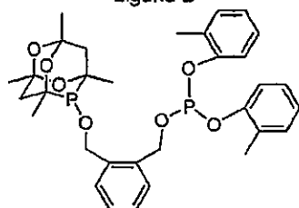
Ligand C
