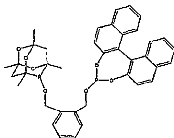
Ligand A
