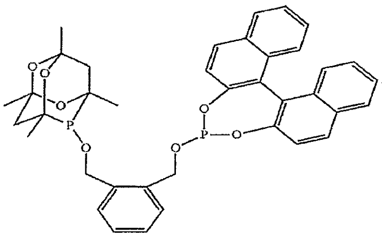
Ligand A
