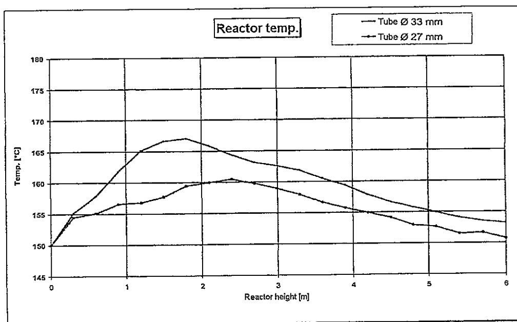
Figure 1: Temperature profile of both reactors after 5 300 h (upper line = tube with diameter 33 mm)
