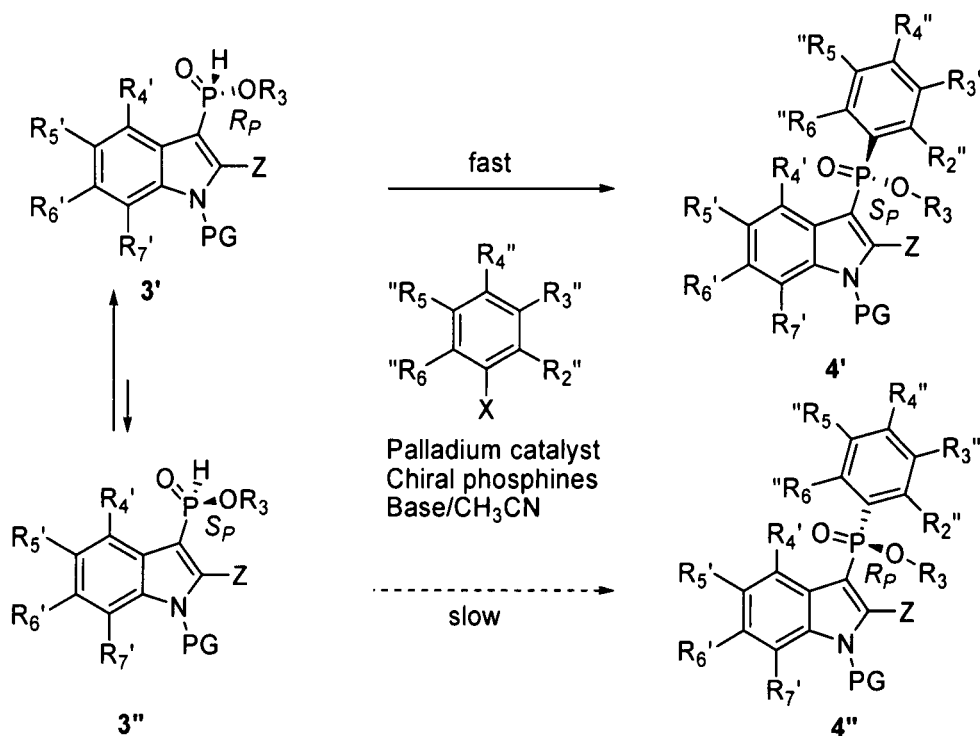
Scheme 8
