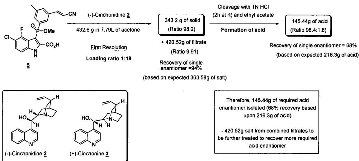
Scheme 17
