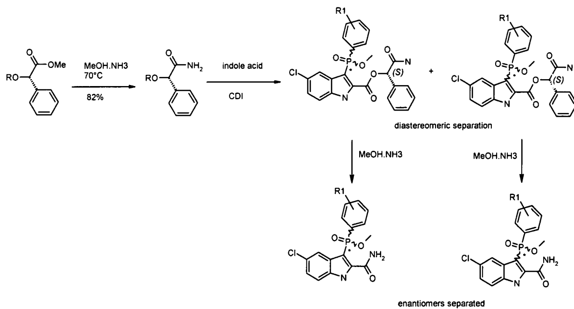
Scheme 27
