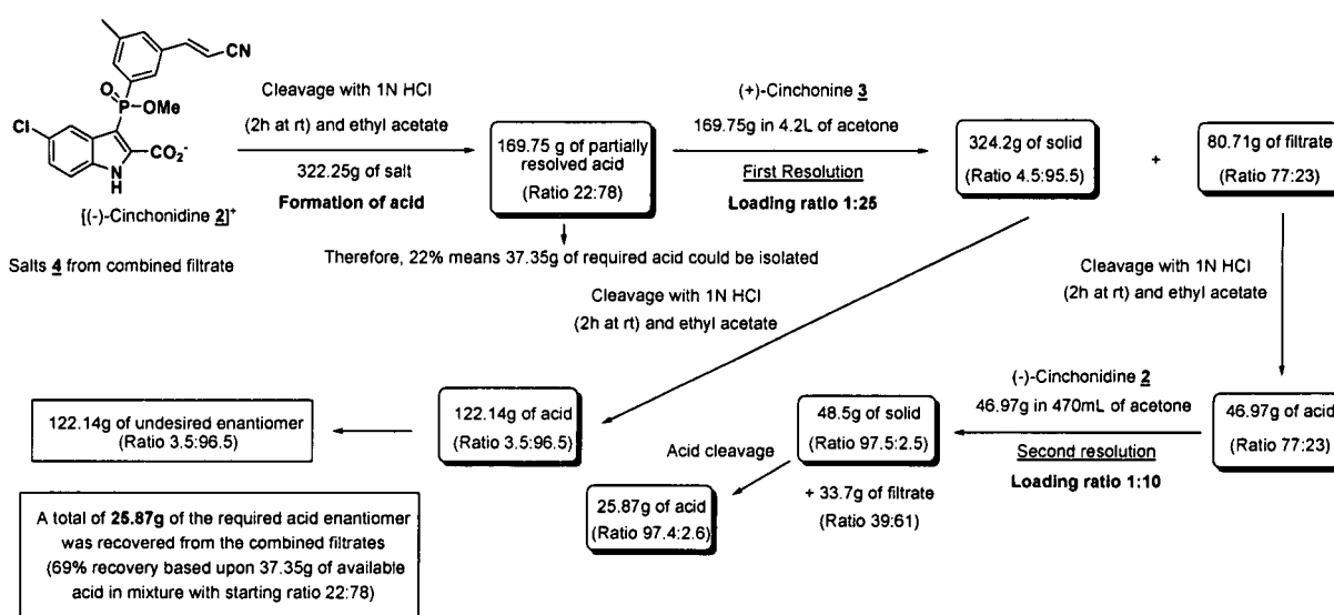
Scheme 16
