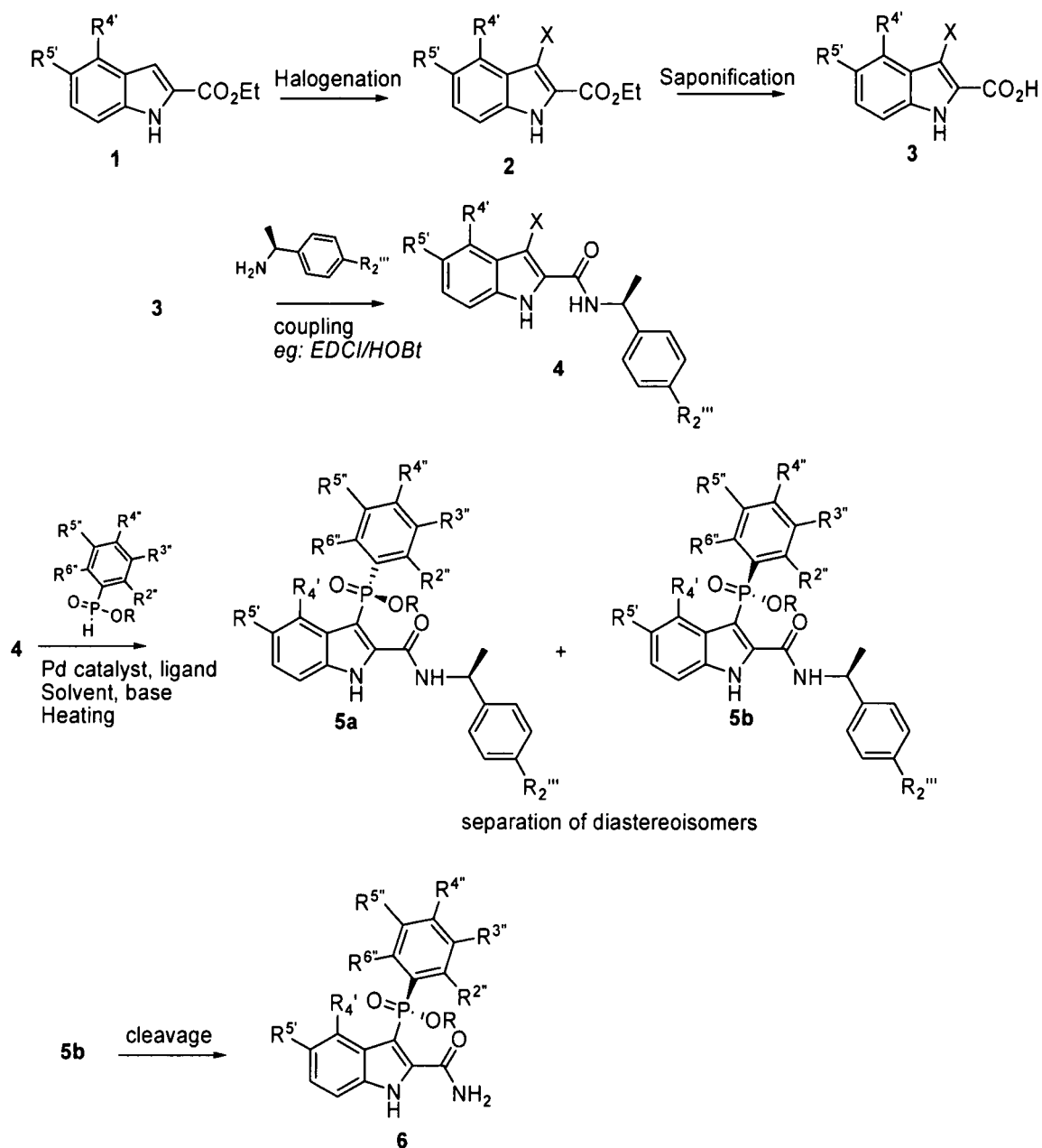
Scheme 13
