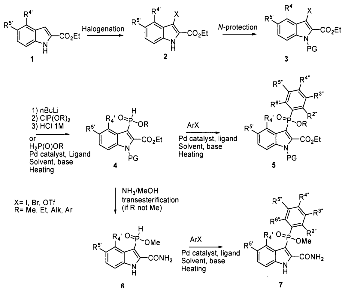
Scheme 5
