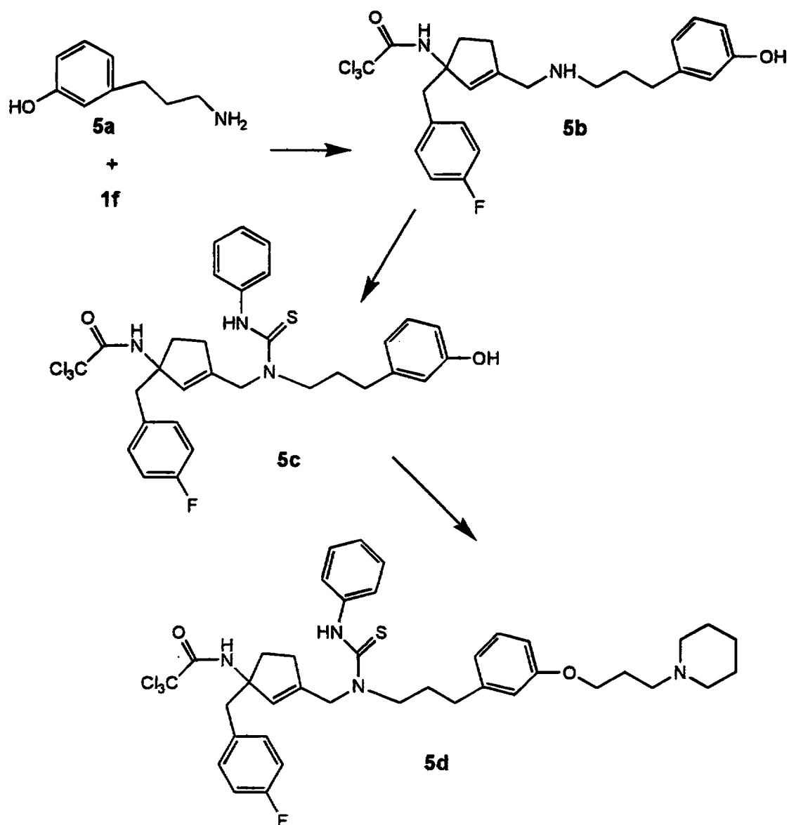
Scheme 5
