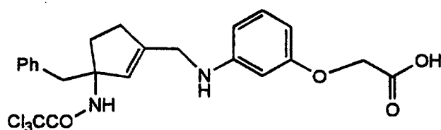
Cpd 45
