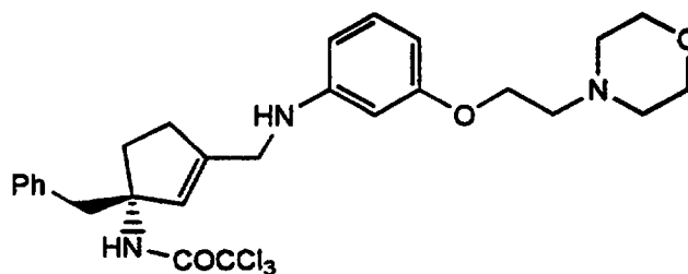
Cpd. 6b
