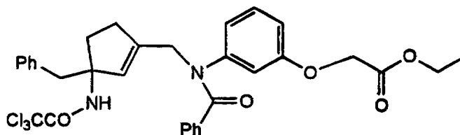
Cpd 46
