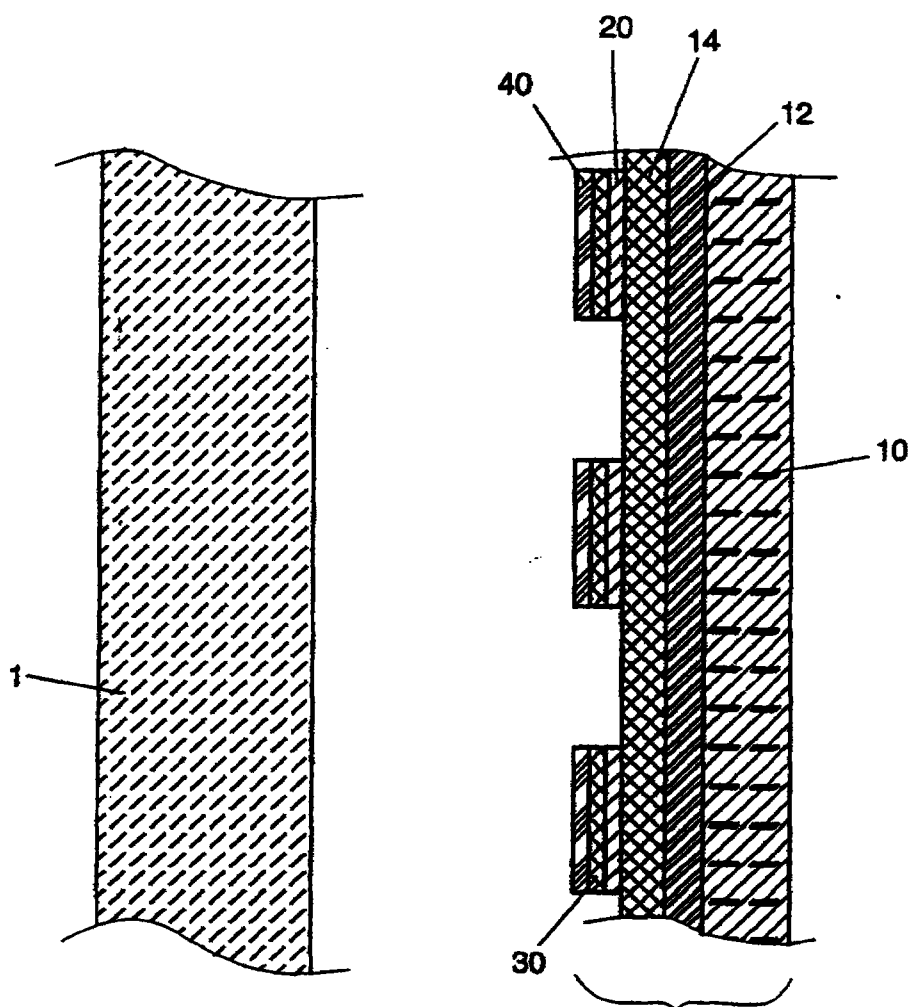
LABEL & SUBSTRATE EXPLODED VIEW
