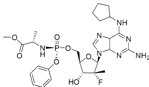
Compound 38
