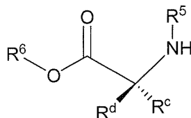
Formula IX
