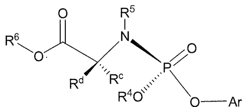
Formula IIIa
