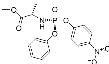
Compound 11
