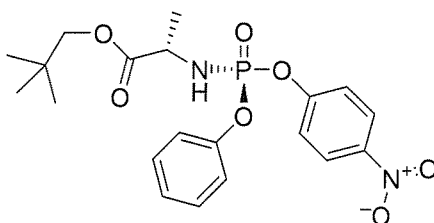
Compound 24
