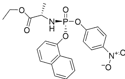
Compound 20
