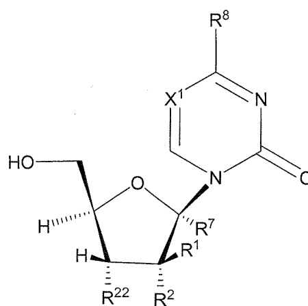
Formula XIV
