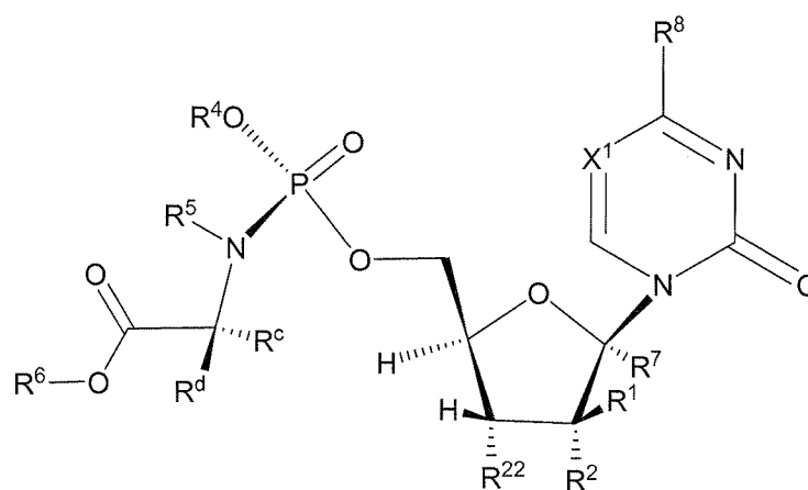
Formula XIIIb
