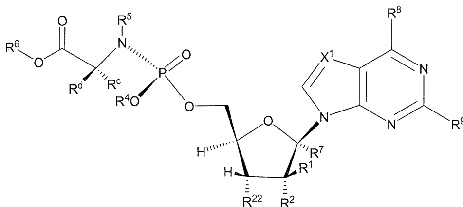
Formula XIa
