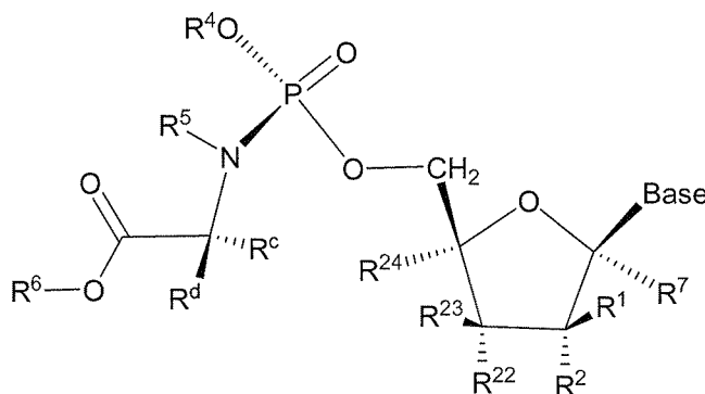
Formula IVb
