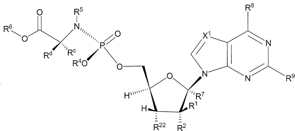
Formula XIa
