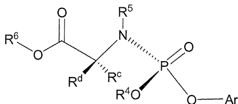
Formula IIIb
