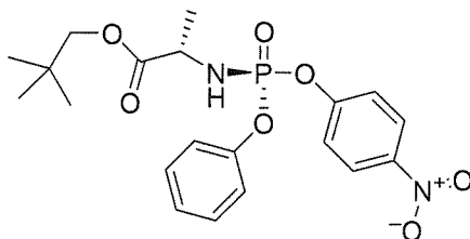
Compound 23
