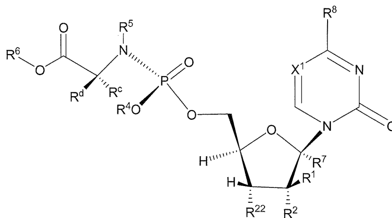
Formula XIIIa
