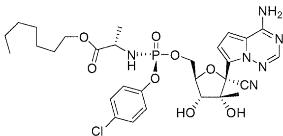
Compound 27
