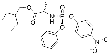
Compound 15
