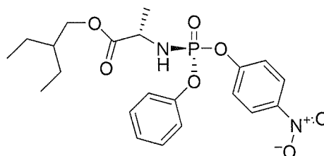
Compound 13
