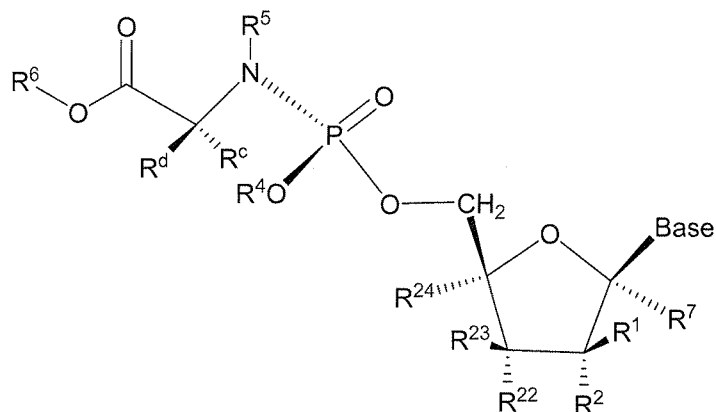
Formula IVa
