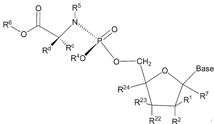
Formula Ia
