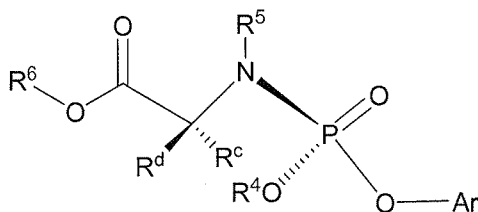
Formula IIIa
