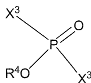
Formula X
