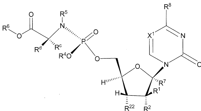
Formula XIIIa
