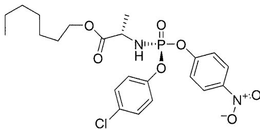
Compound 19
