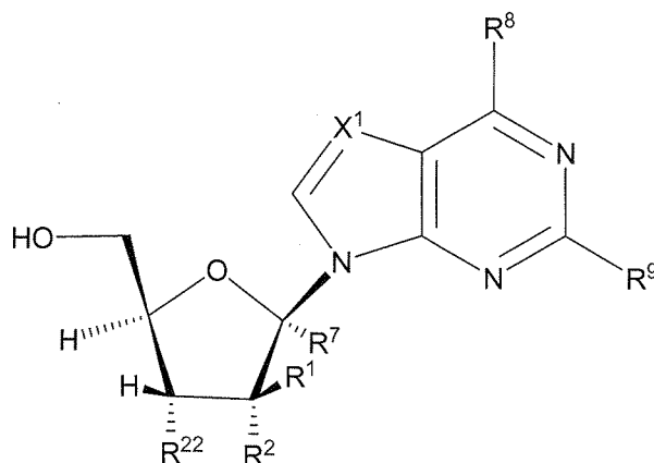
Formula XII
