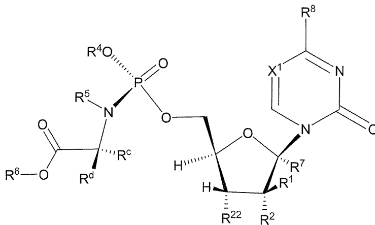
Formula XIIIb
