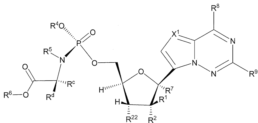
Formula VIb
