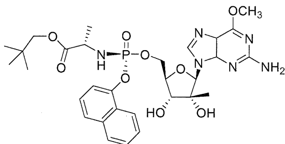
Compound 36
