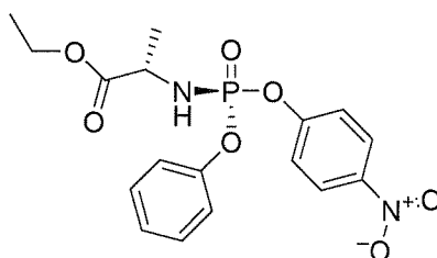
Compound 12
