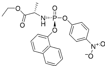
Compound 21
