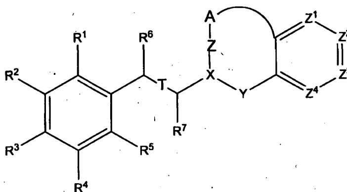
Formula (IV)
