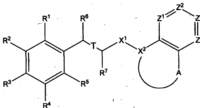
Formula (III)
