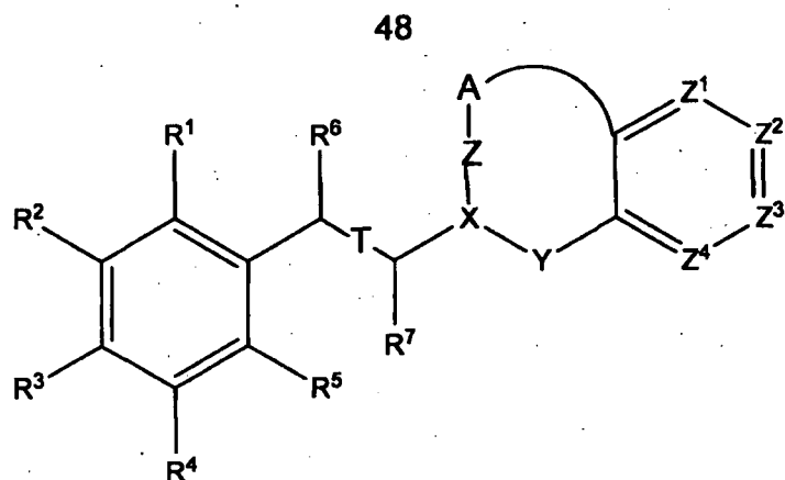
Formula (IV)
