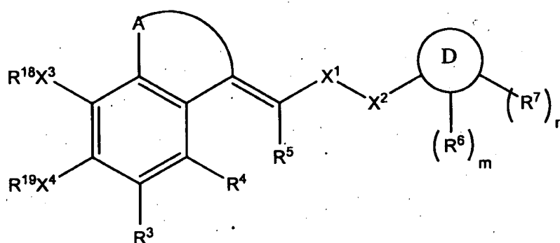
Formula (IIa)
