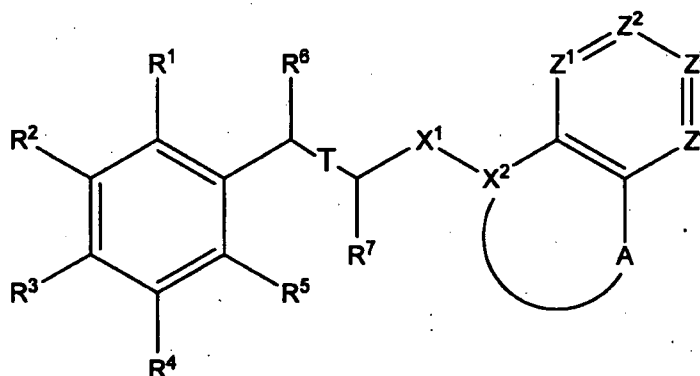
Formula (III)
