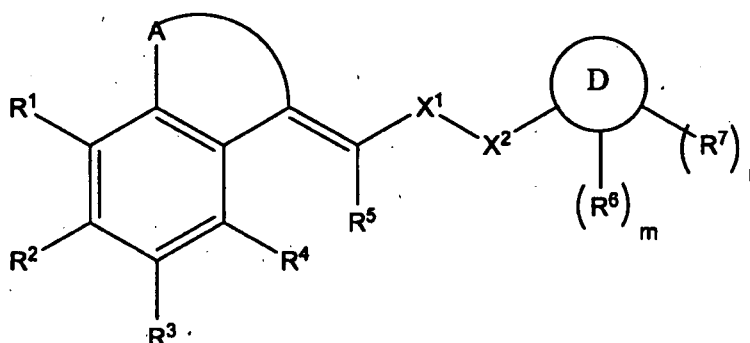
Formula (II)
