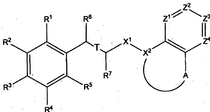
Formula (III)
