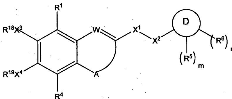
Formula (Ia)
