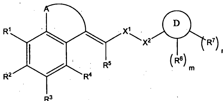
Formula (II)
