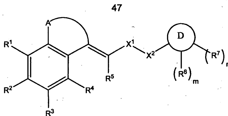
Formula (II)
