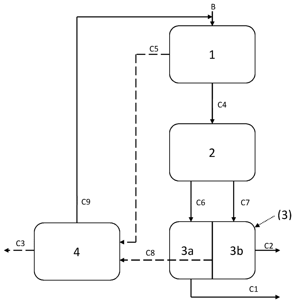
Figure 1: Preferred configuration of optical sorters in step c)
