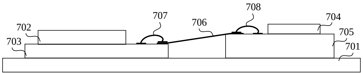
Optoelectronic apparatus 700
