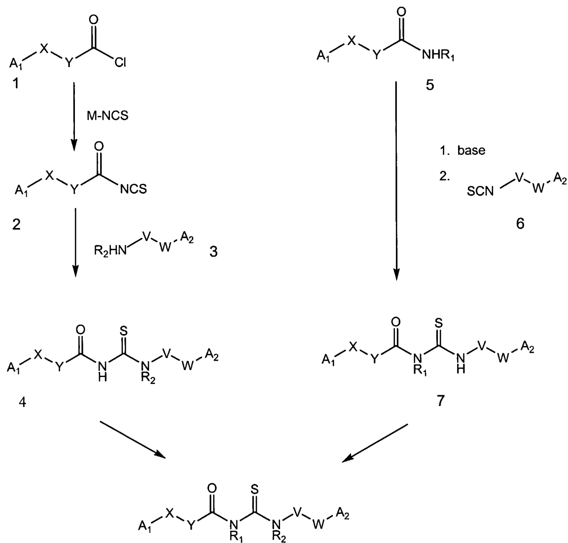
Scheme I
