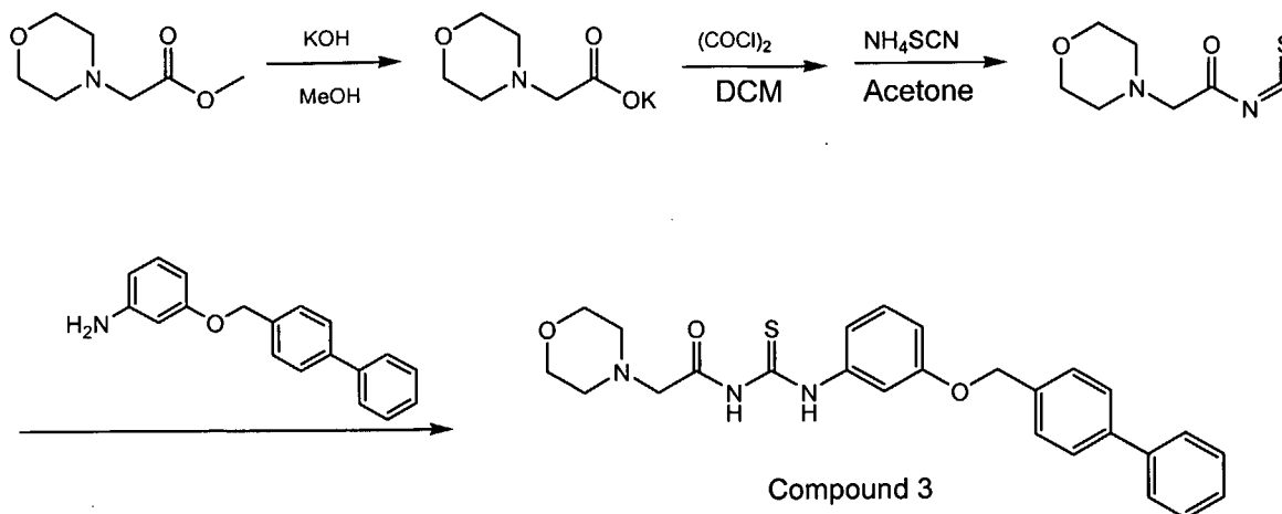
Scheme 2. Synthesis of 1-[3-(Biphenyl-4-ylmethoxy)-phenyl]-3-(2-morpholin-4-yl-acetyl)-thiourea
