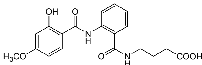
(compound 13)
