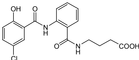
(compound 19)
