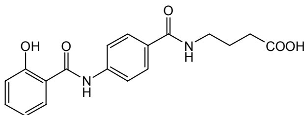
(compound 1)
