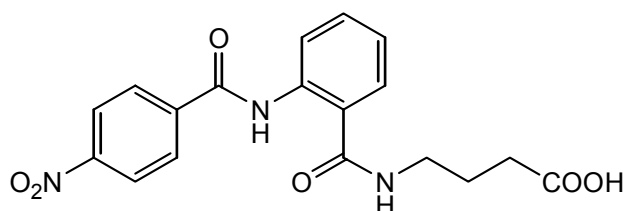
(compound 15)
