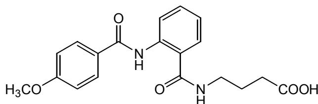
(compound 16)
