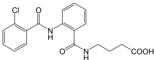
(compound 20)
