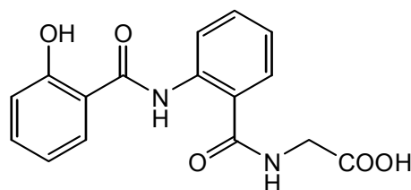
(compound 10)
