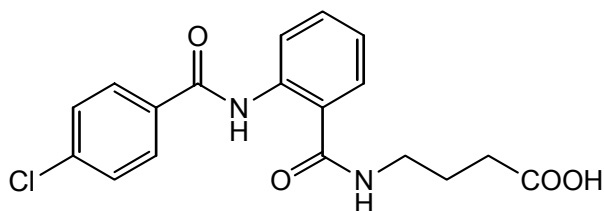
(compound 17)
