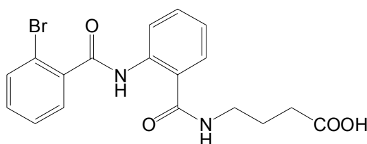
(compound 21)
