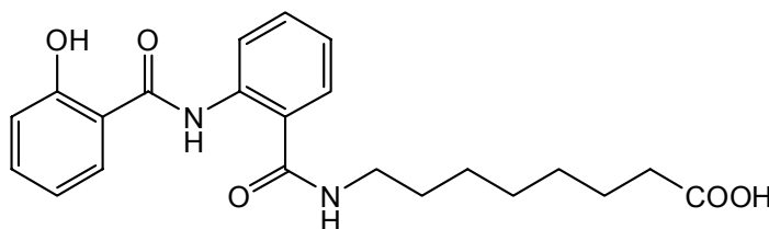
(compound 6)
