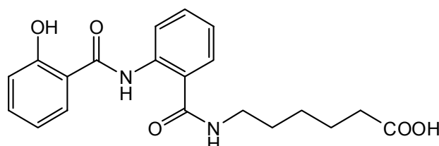
(compound 7)
