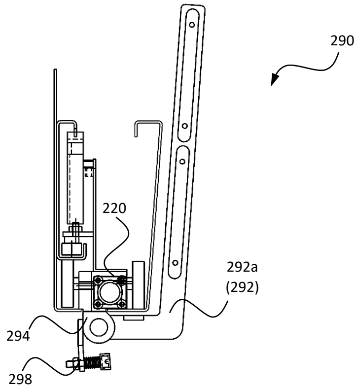
Fig. 12C (VIEW B-B)
