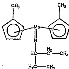
Compound No.29
