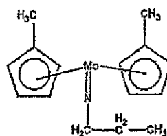
Compound No.24
