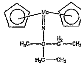
Compound No.12
