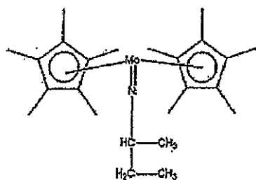
Compound No.47
