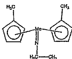
Compound No.23
