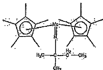
Compound No.51
