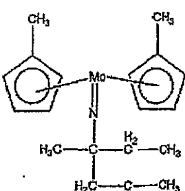
Compound No.37
