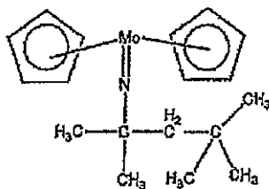
Compound No.19
