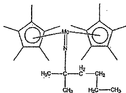
Compound No.55
