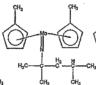
Compound No.35
