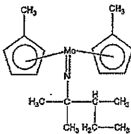
Compound No.39
