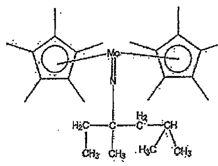
Compound No.63
