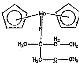
Compound No.16
