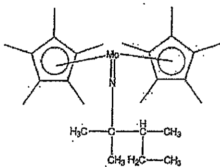
Compound No.60
