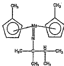
Compound No.32
