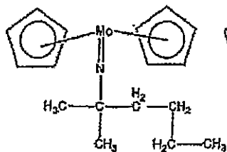
Compound No.13
