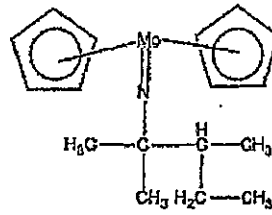
Compound No.18
