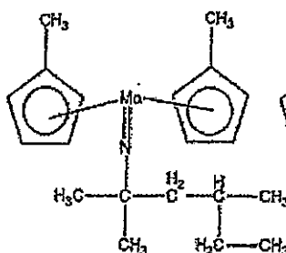
Compound No.41
