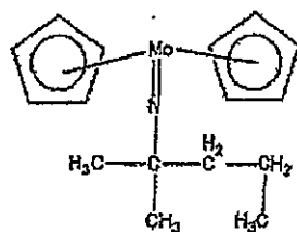
Compound No.10
