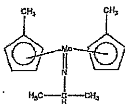
Compound No.25
