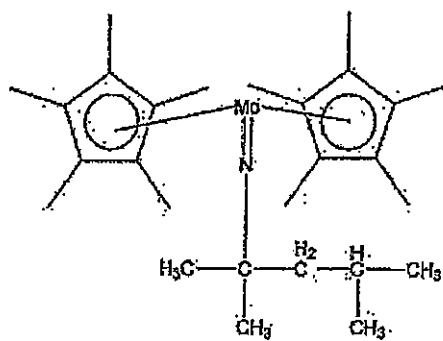
Compound No.56
