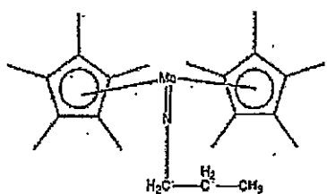
Compound No.45
