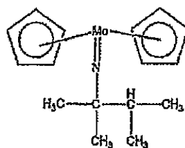
Compound No.11
