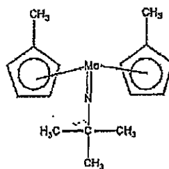
Compound No.27
