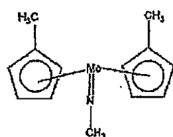
Compound No.22
