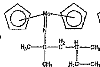
Compound No.20
