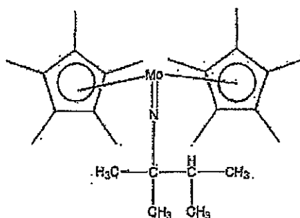
Compound No.53
