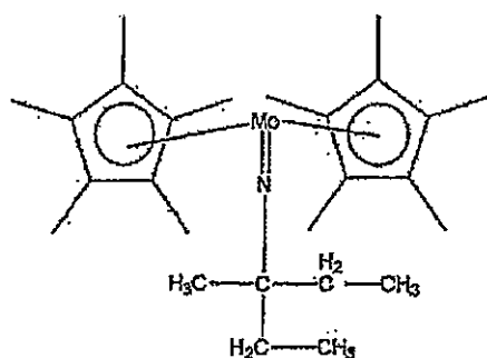
Compound No.54
