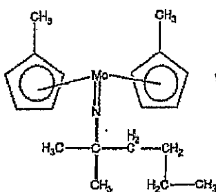
Compound No.34
