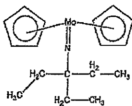
Compound No.17
