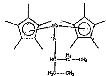
Compound No.50
