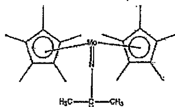
Compound No.46
