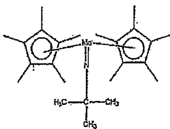
Compound No.48
