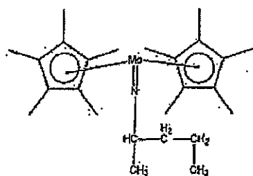
Compound No.49
