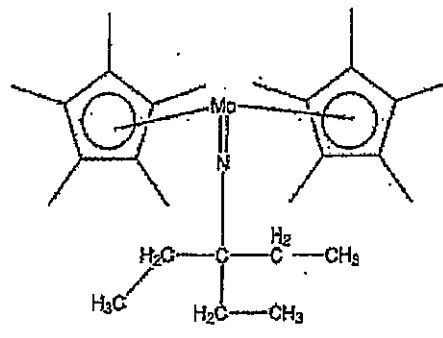
Compound No.59
