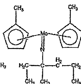
Compound No.36
