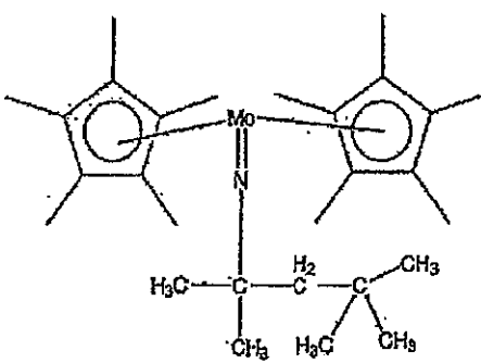
Compound No.61
