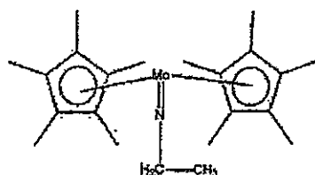
Compound No.44
