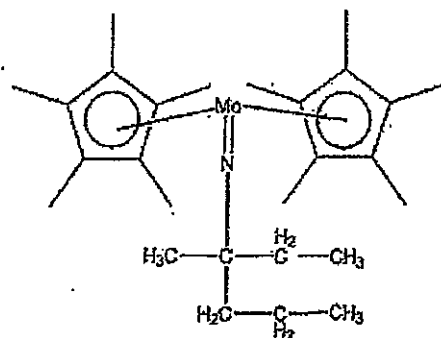
Compound No.58
