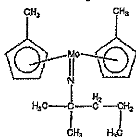
Compound No.31
