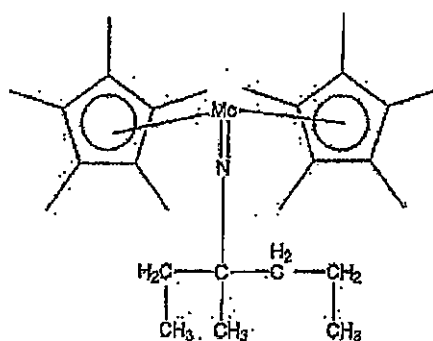
Compound No.57
