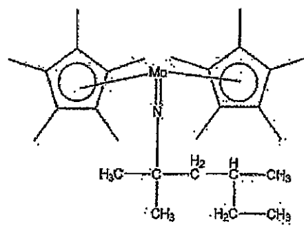
Compound No.62
