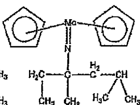
Compound No.21
