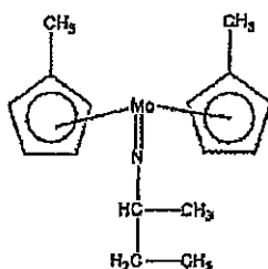
Compound No.26
