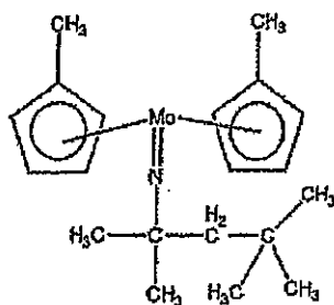
Compound No.40
