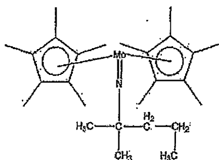
Compound No.52
