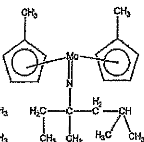
Compound No.42
