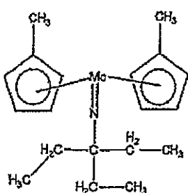
Compound No.38
