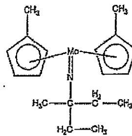
Compound No.33
