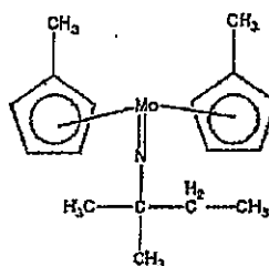
Compound No.30
