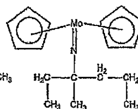
Compound No.15
