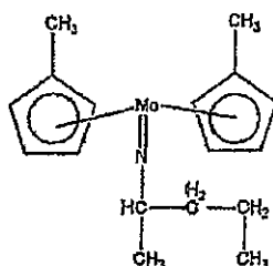
Compound No.28
