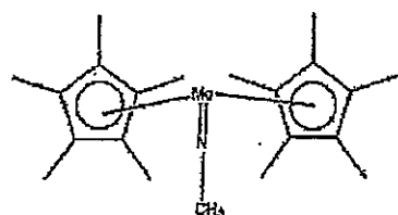
Compound No.43
