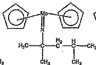
Compound No.14
