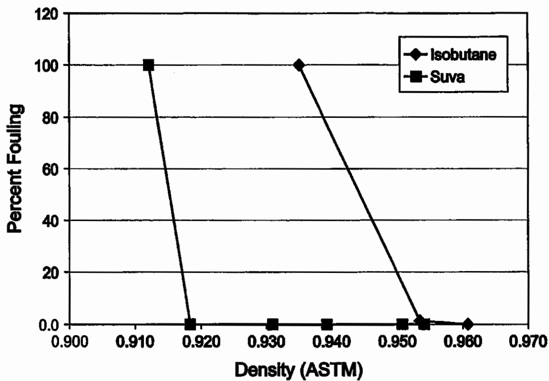
Fig. 1 Fouling vs. Density (at 107.8°C)
