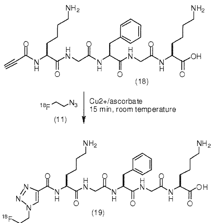
Reaction Scheme 7
