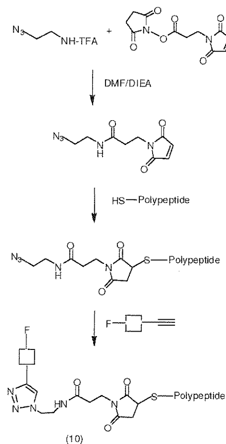
Reaction Scheme 4
