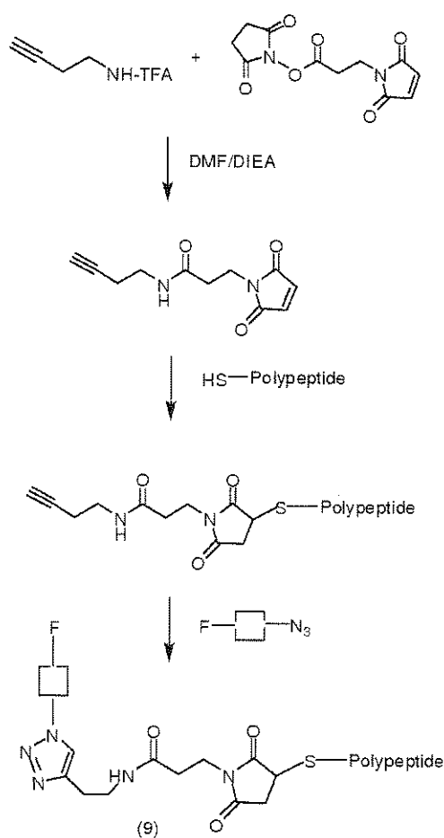
Reaction Scheme 3
