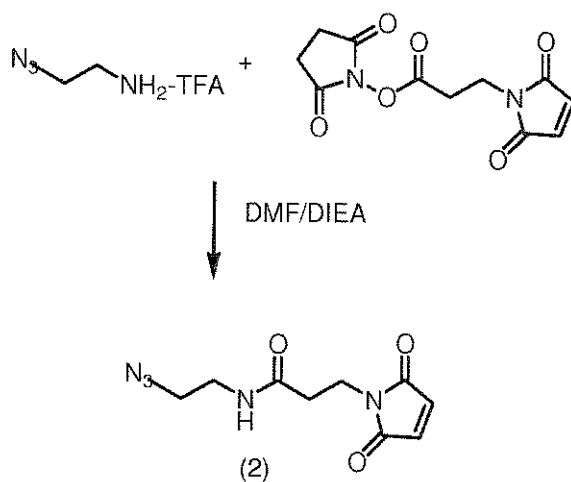
Reaction Scheme 2
