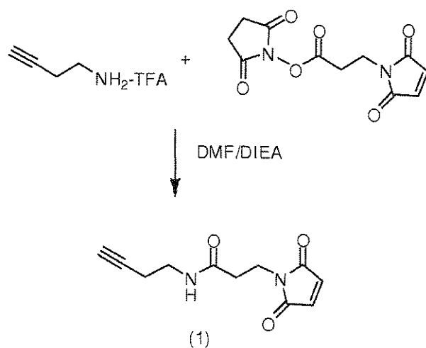
Reaction Scheme 1
