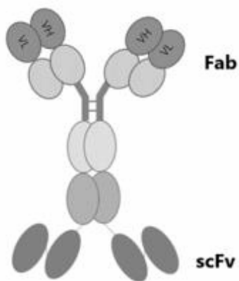
D-symmetric scFv bispecific antibody
