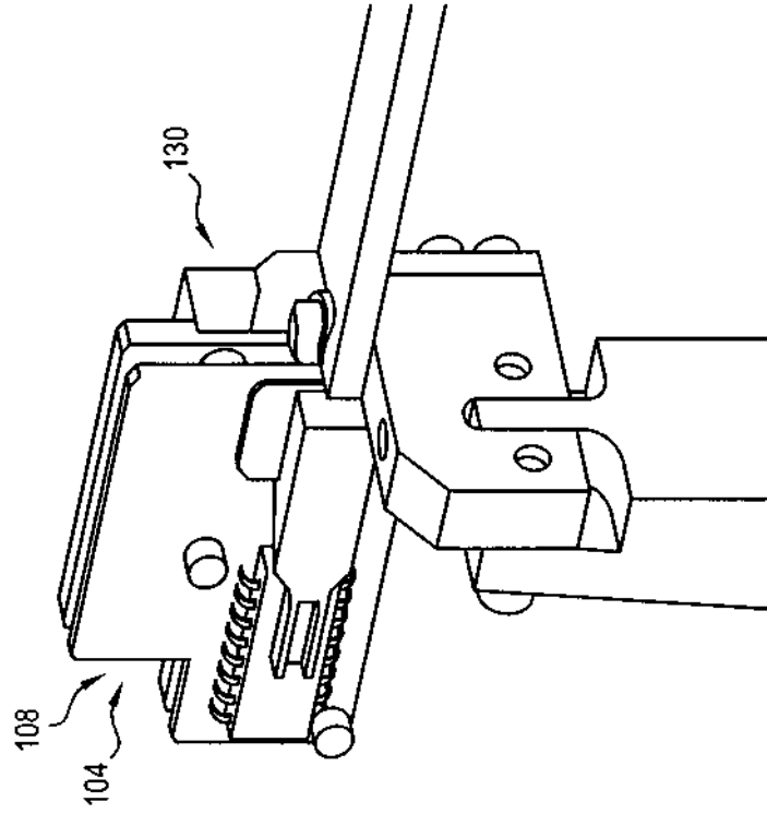
90 Degree Mount (Horizontal Scan)
