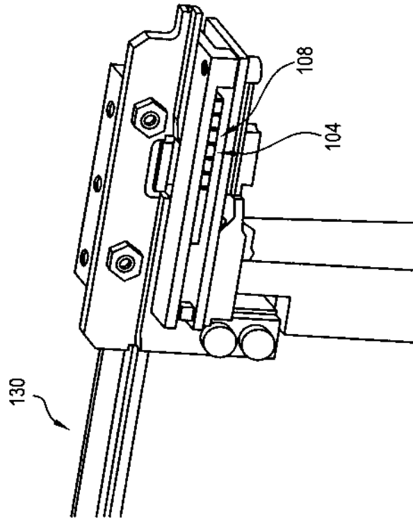
0 Degree Mount (Vertical Scan)
