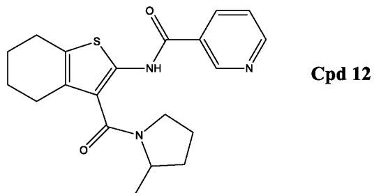
N-(3-(2-methylpyrrolidine-1-carbonyl)- 4,5,6,7-tetrahydrobenzo[b]thiophen-2- yl)nicotinamide
