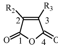
maleic anhydride system
