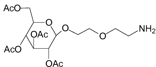
Glc \beta -isomer
