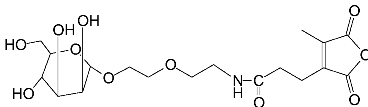
Man \alpha -isomer
