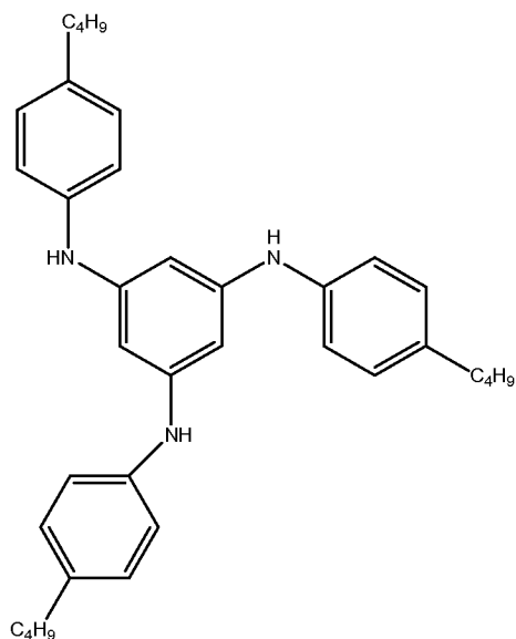
Formula IV
