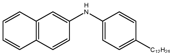
Formula VI
