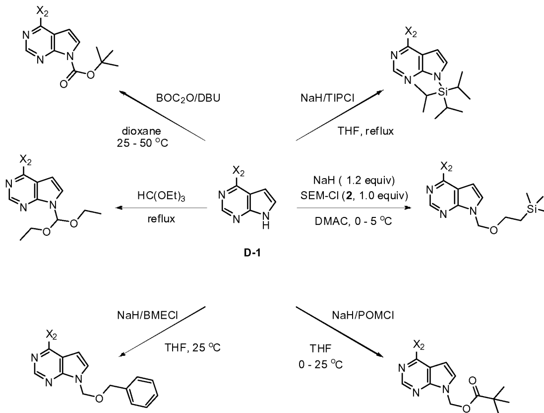
Scheme 13
