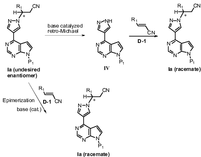
Scheme 8
