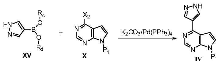
Scheme 10
