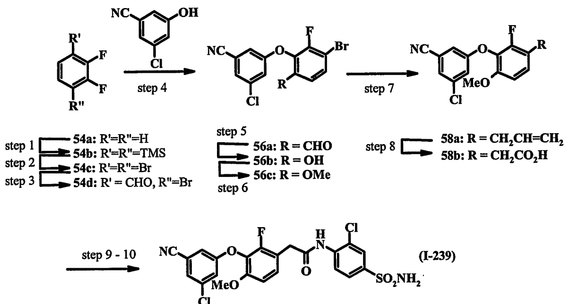
SCHEME 7
