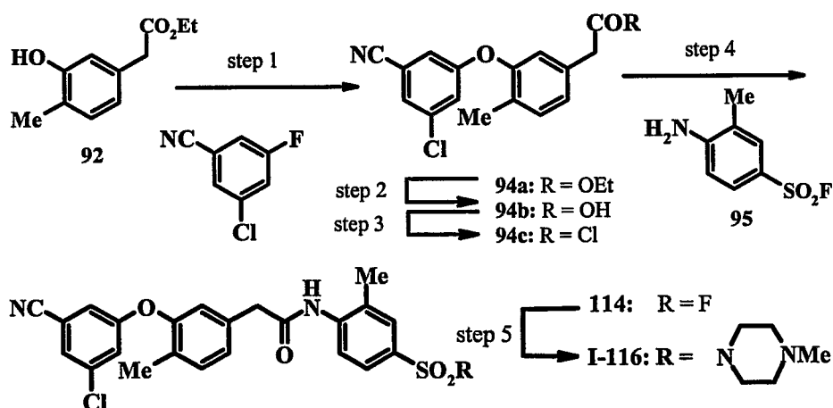
15 SCHEME 12
