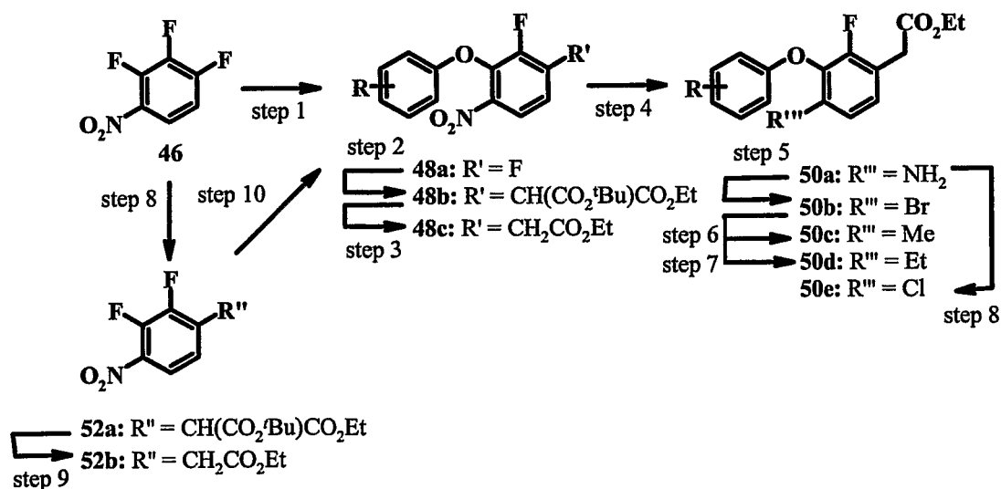
SCHEME 6
