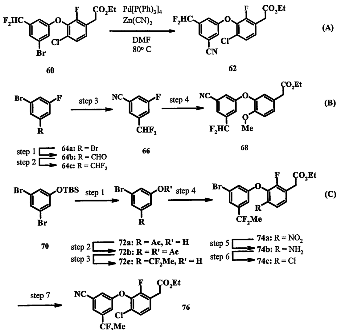
10 SCHEME 8
